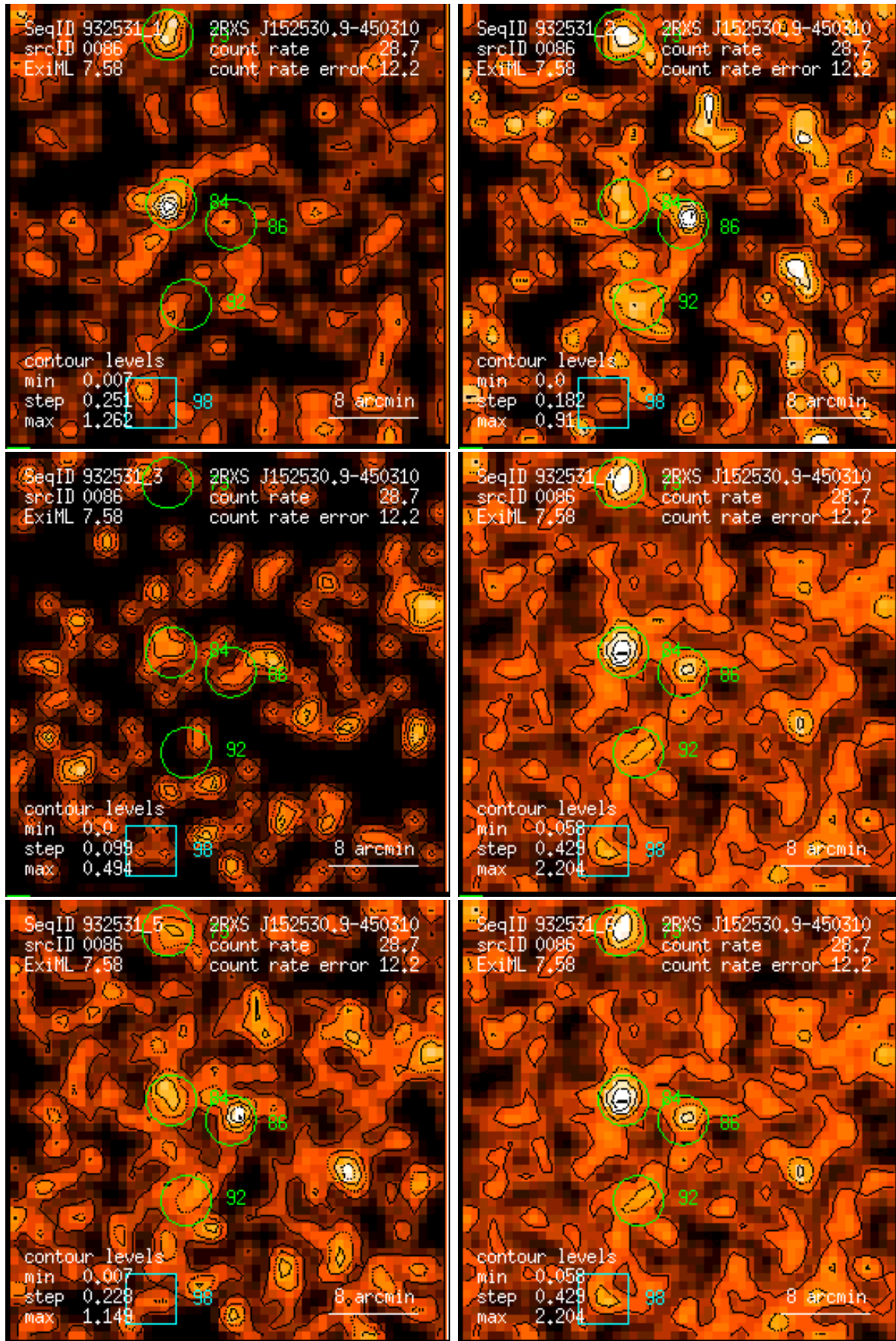
Figure 86: RASS 932531: detection 0086: band rate images, Gaussian filter: (1) PSPC channels 11 – 41, (2) 52 – 90, (3) 91 – 201, (4) 11 – 235, (5) 52 – 201, (6) 11 – 201. Broad band rates in counts/ks. Band rate contour levels in counts/ks/arcmin 2 .
