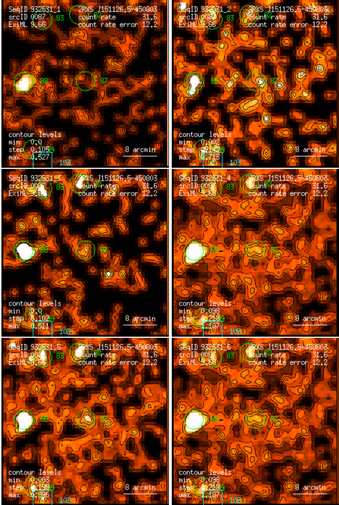
Figure 87: RASS 932531: detection 0087: band rate images, Gaussian filter: (1) PSPC channels 11 – 41, (2) 52 – 90, (3) 91 – 201, (4) 11 – 235, (5) 52 – 201, (6) 11 – 201. Broad band rates in counts/ks. Band rate contour levels in counts/ks/arcmin 2 .
