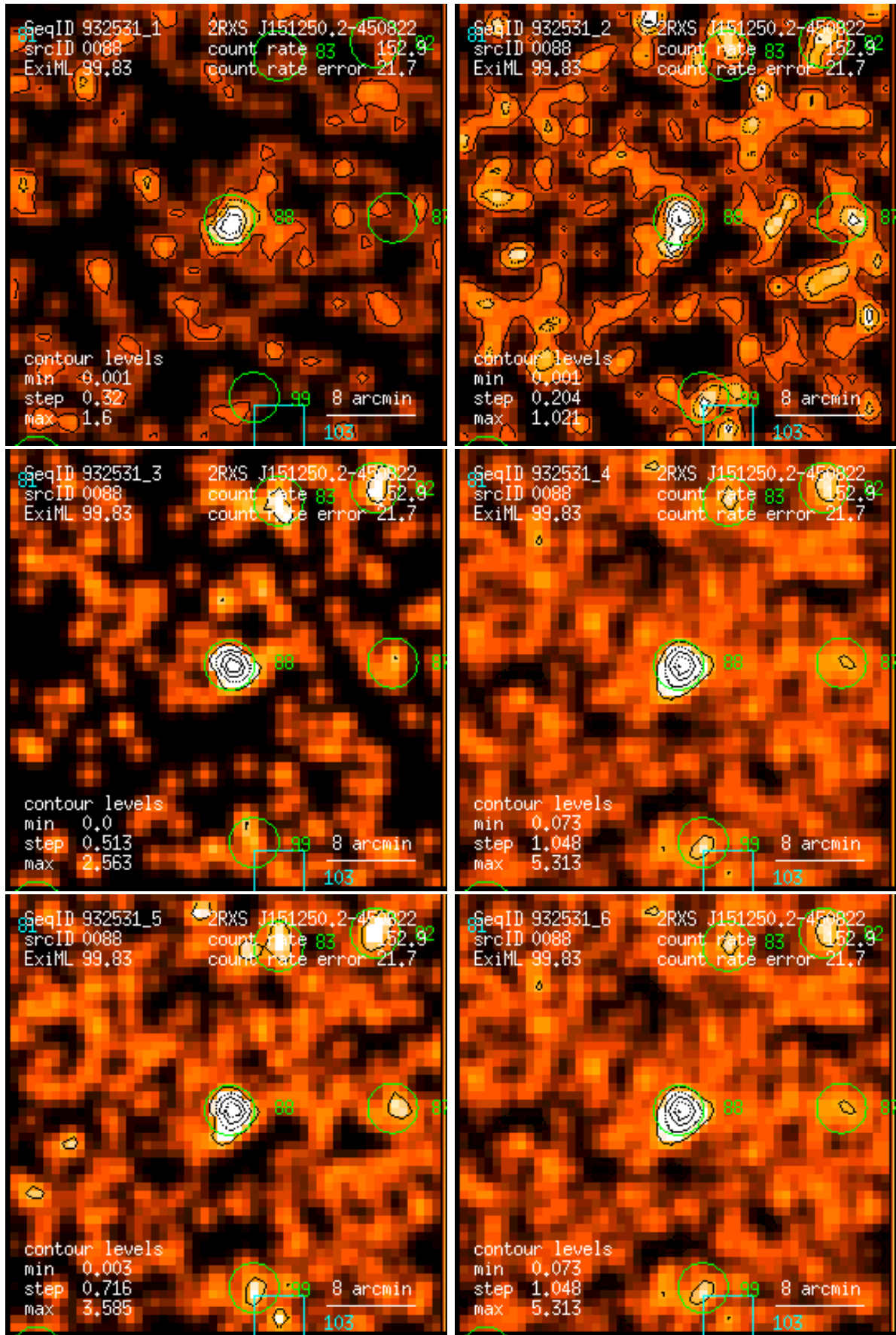
Figure 88: RASS 932531: detection 0088: band rate images, Gaussian filter: (1) PSPC channels 11 – 41, (2) 52 – 90, (3) 91 – 201, (4) 11 – 235, (5) 52 – 201, (6) 11 – 201. Broad band rates in counts/ks. Band rate contour levels in counts/ks/arcmin 2 .
