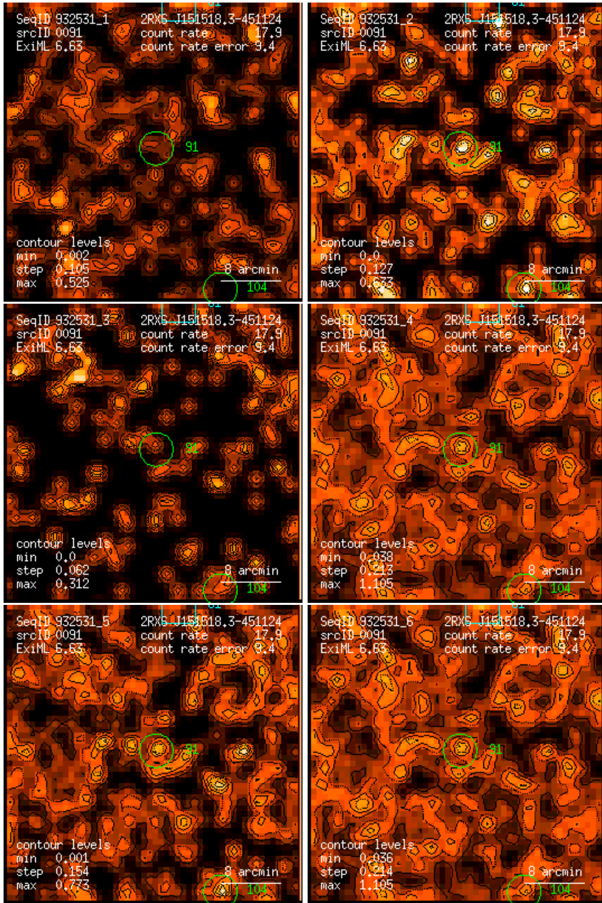
Figure 91: RASS 932531: detection 0091: band rate images, Gaussian filter: (1) PSPC channels 11 – 41, (2) 52 – 90, (3) 91 – 201, (4) 11 – 235, (5) 52 – 201, (6) 11 – 201. Broad band rates in counts/ks. Band rate contour levels in counts/ks/arcmin 2 .
