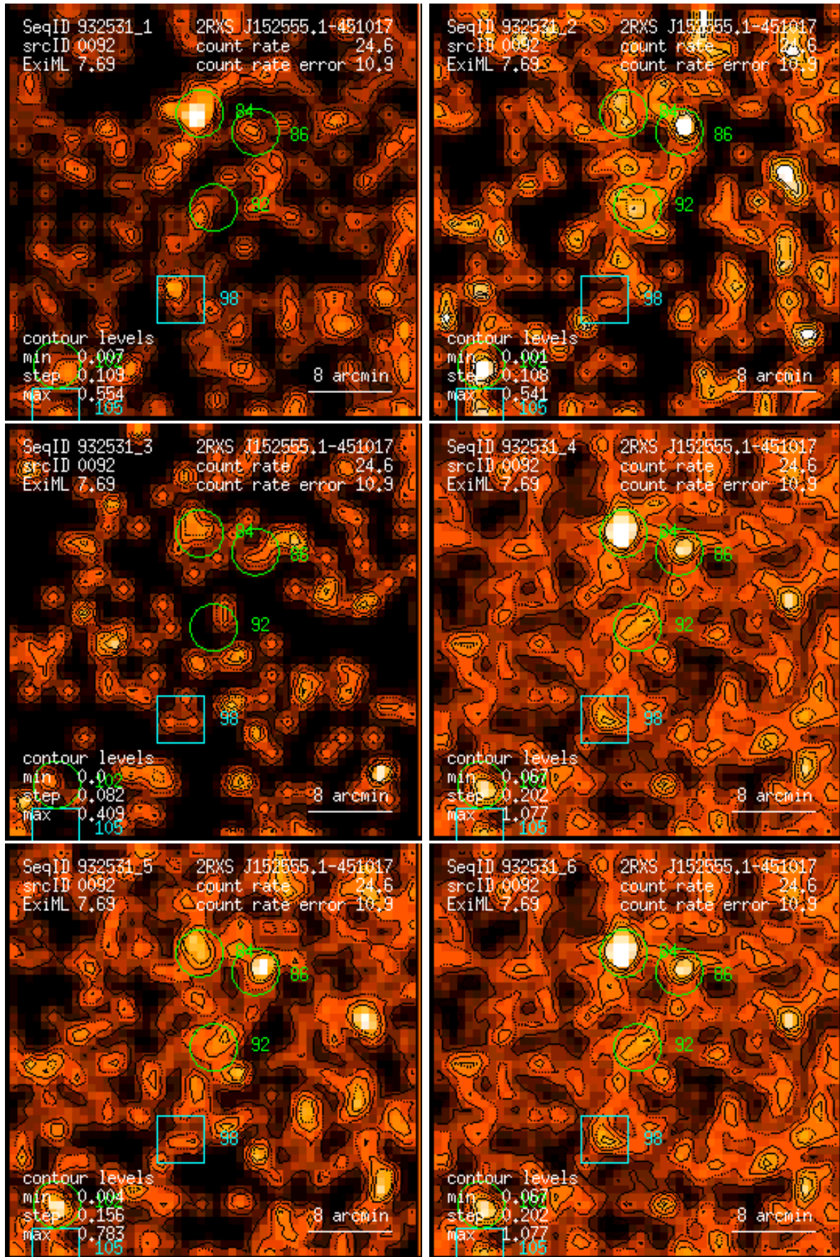
Figure 92: RASS 932531: detection 0092: band rate images, Gaussian filter: (1) PSPC channels 11 – 41, (2) 52 – 90, (3) 91 – 201, (4) 11 – 235, (5) 52 – 201, (6) 11 – 201. Broad band rates in counts/ks. Band rate contour levels in counts/ks/arcmin 2 .
