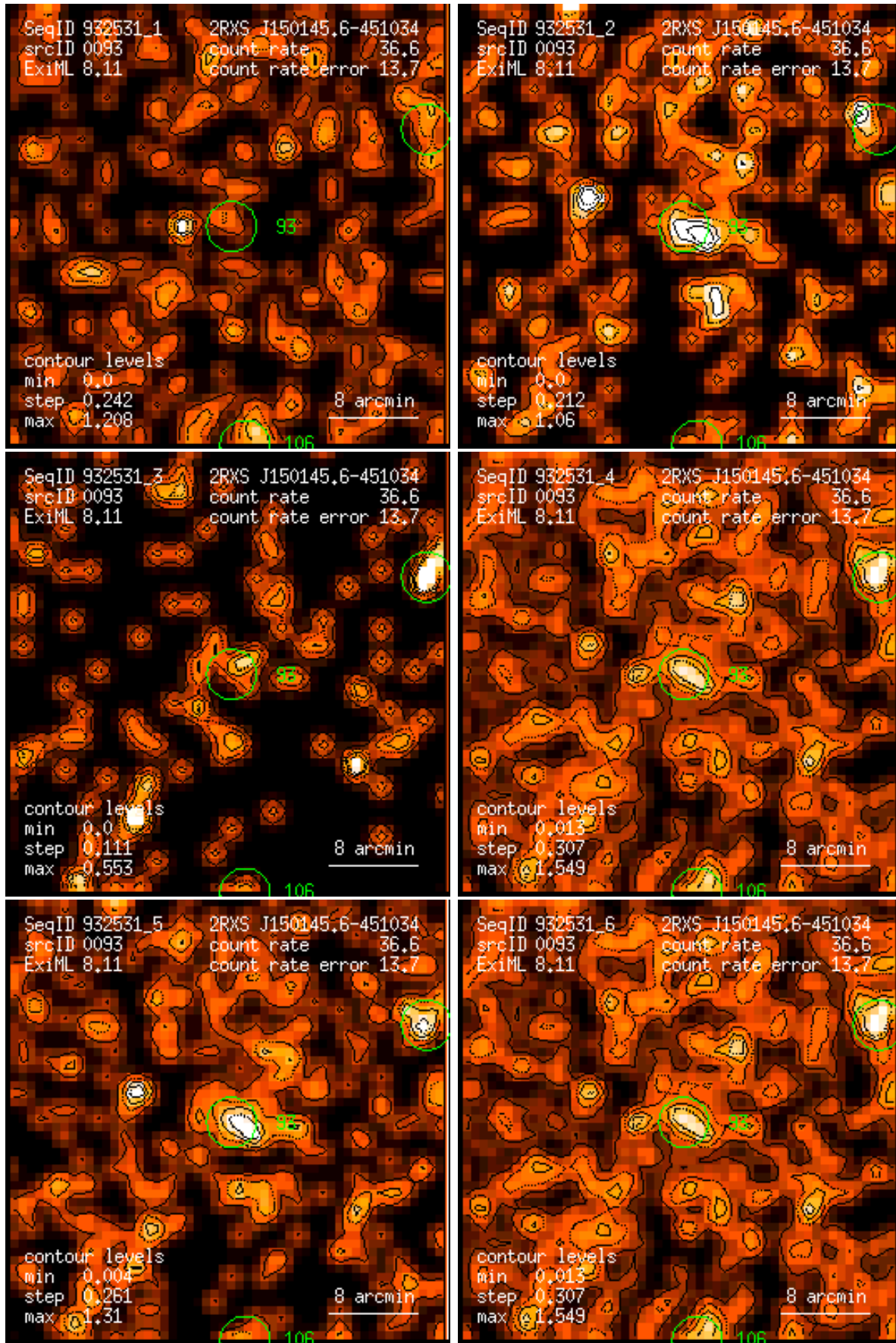
Figure 93: RASS 932531: detection 0093: band rate images, Gaussian filter: (1) PSPC channels 11 – 41, (2) 52 – 90, (3) 91 – 201, (4) 11 – 235, (5) 52 – 201, (6) 11 – 201. Broad band rates in counts/ks. Band rate contour levels in counts/ks/arcmin 2 .
