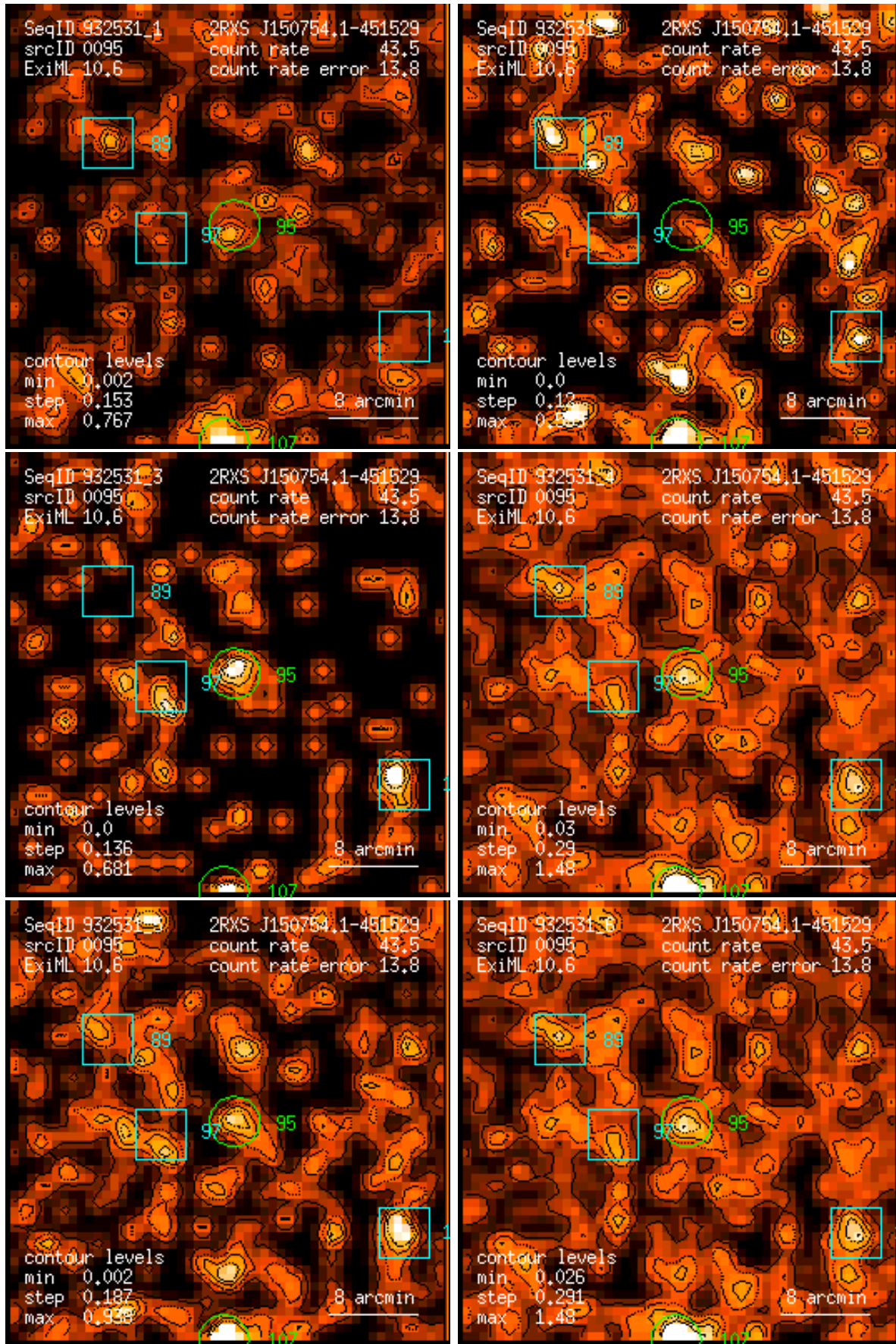
Figure 95: RASS 932531: detection 0095: band rate images, Gaussian filter: (1) PSPC channels 11 – 41, (2) 52 – 90, (3) 91 – 201, (4) 11 – 235, (5) 52 – 201, (6) 11 – 201. Broad band rates in counts/ks. Band rate contour levels in counts/ks/arcmin 2 .
