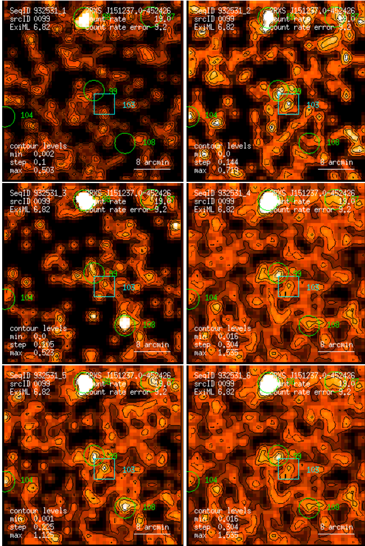
Figure 99: RASS 932531: detection 0099: band rate images, Gaussian filter: (1) PSPC channels 11 – 41, (2) 52 – 90, (3) 91 – 201, (4) 11 – 235, (5) 52 – 201, (6) 11 – 201. Broad band rates in counts/ks. Band rate contour levels in counts/ks/arcmin 2 .
