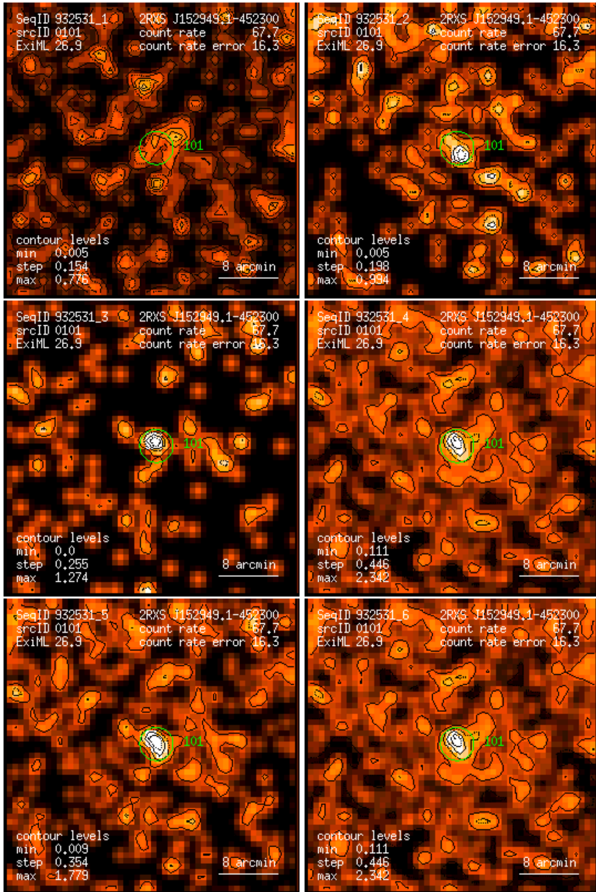
Figure 101: RASS 932531: detection 0101: band rate images, Gaussian filter: (1) PSPC channels 11 – 41, (2) 52 – 90, (3) 91 – 201, (4) 11 – 235, (5) 52 – 201, (6) 11 – 201. Broad band rates in counts/ks. Band rate contour levels in counts/ks/arcmin 2 .
