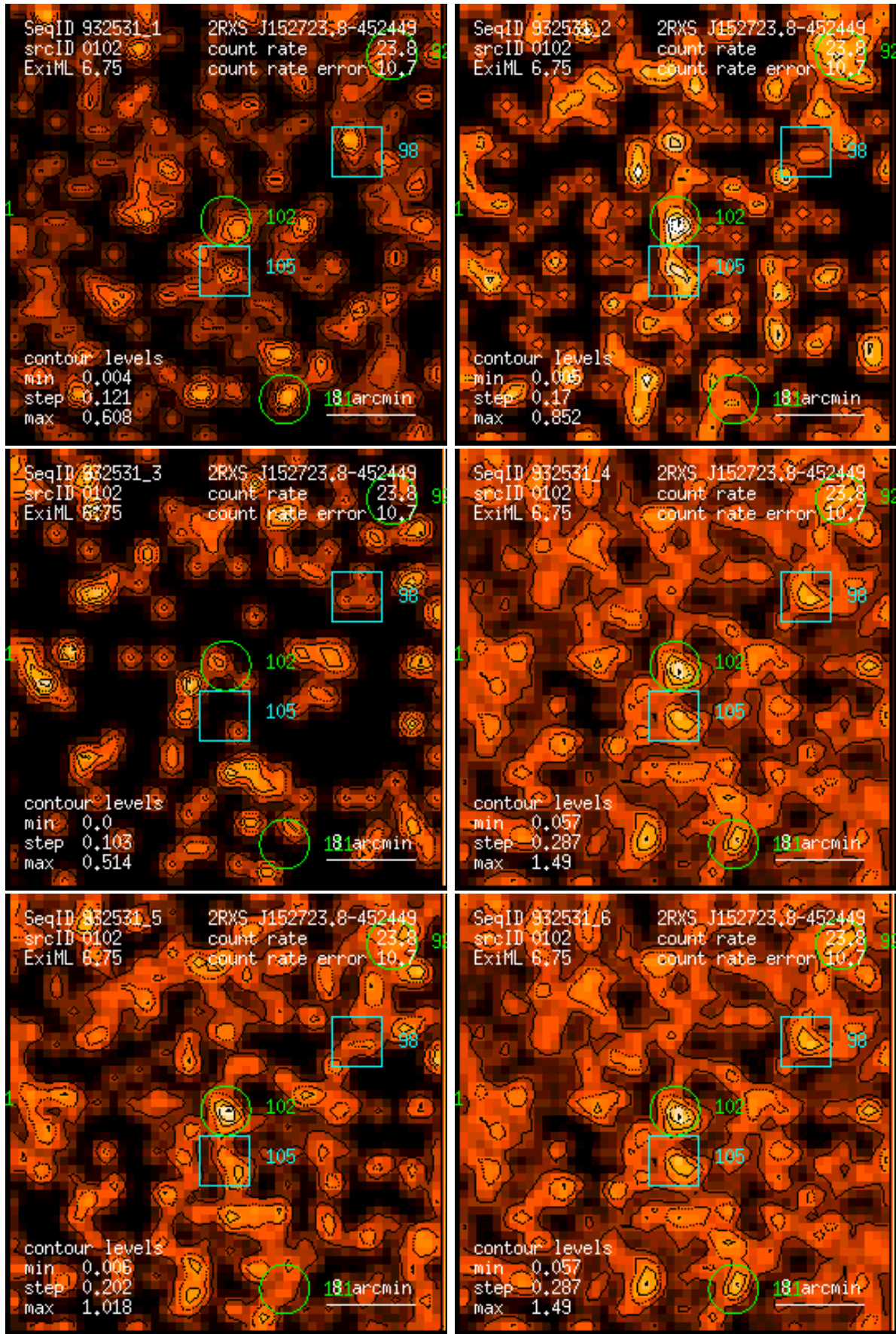
Figure 102: RASS 932531: detection 0102: band rate images, Gaussian filter: (1) PSPC channels 11 – 41, (2) 52 – 90, (3) 91 – 201, (4) 11 – 235, (5) 52 – 201, (6) 11 – 201. Broad band rates in counts/ks. Band rate contour levels in counts/ks/arcmin 2 .
