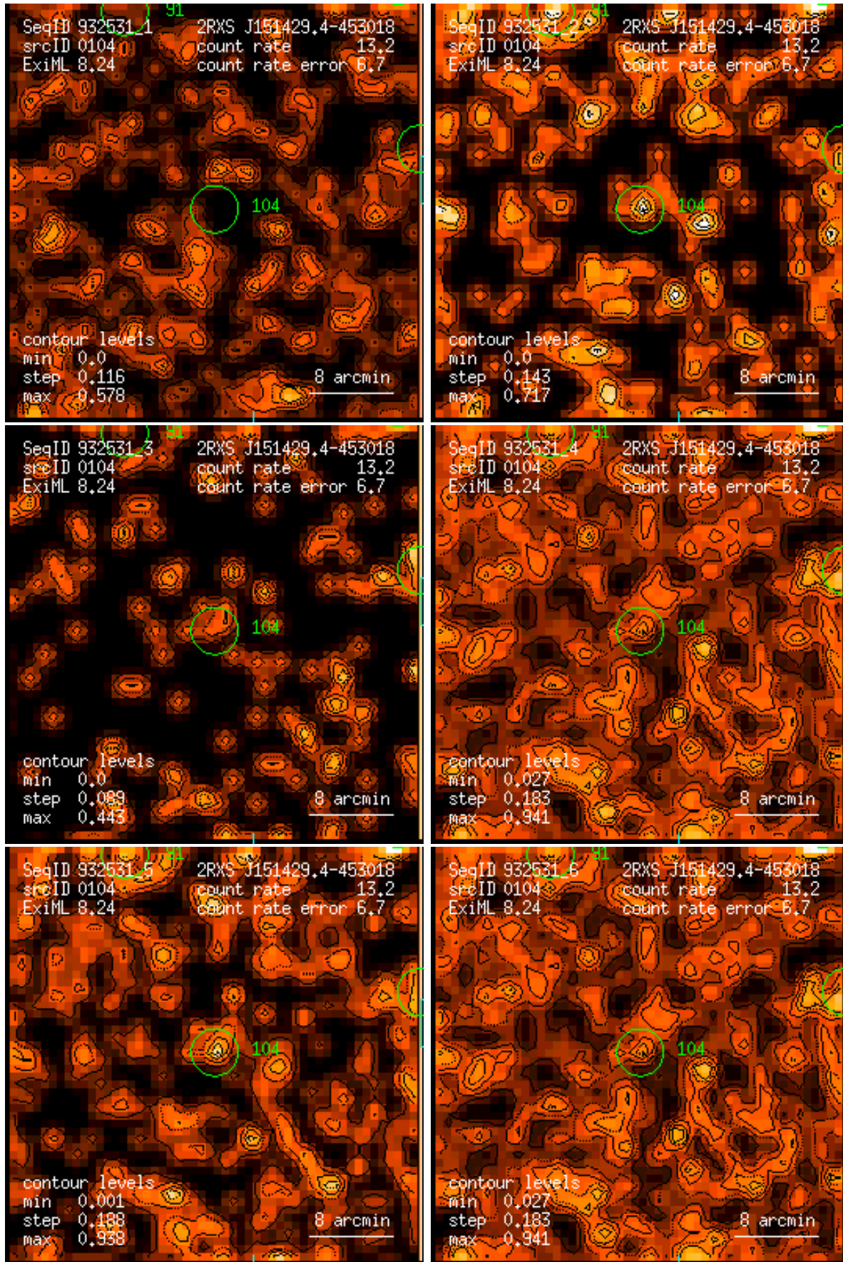
Figure 104: RASS 932531: detection 0104: band rate images, Gaussian filter: (1) PSPC channels 11 – 41, (2) 52 – 90, (3) 91 – 201, (4) 11 – 235, (5) 52 – 201, (6) 11 – 201. Broad band rates in counts/ks. Band rate contour levels in counts/ks/arcmin 2 .
