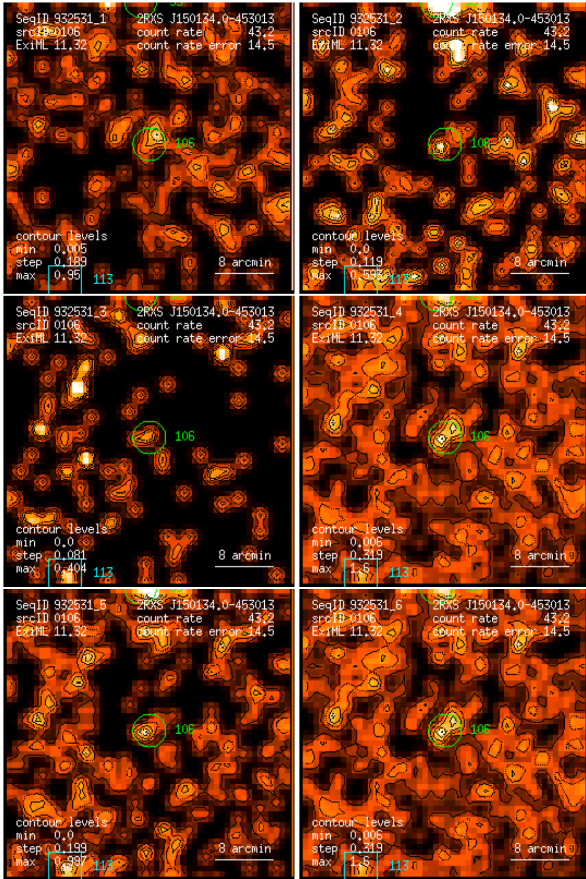
Figure 106: RASS 932531: detection 0106: band rate images, Gaussian filter: (1) PSPC channels 11 – 41, (2) 52 – 90, (3) 91 – 201, (4) 11 – 235, (5) 52 – 201, (6) 11 – 201. Broad band rates in counts/ks. Band rate contour levels in counts/ks/arcmin 2 .
