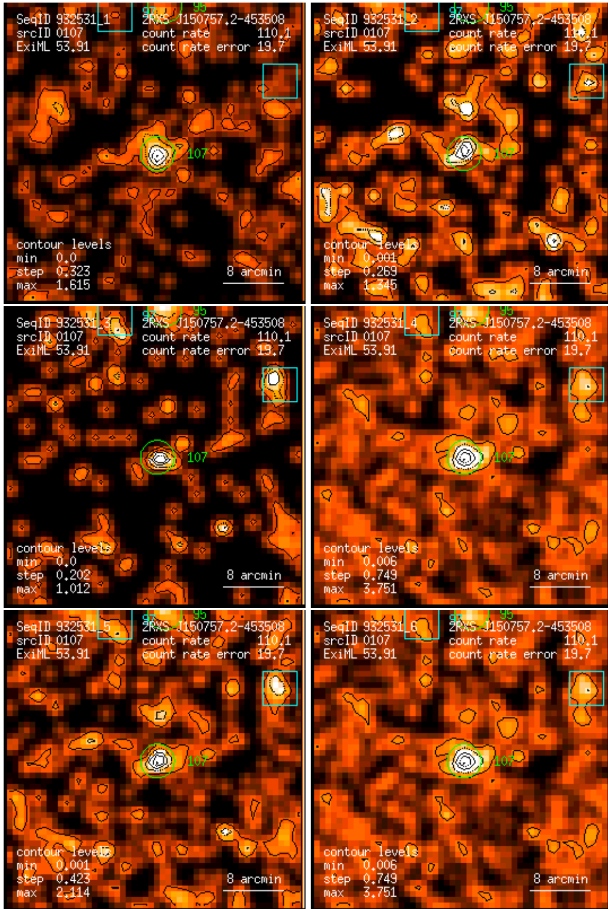
Figure 107: RASS 932531: detection 0107: band rate images, Gaussian filter: (1) PSPC channels 11 – 41, (2) 52 – 90, (3) 91 – 201, (4) 11 – 235, (5) 52 – 201, (6) 11 – 201. Broad band rates in counts/ks. Band rate contour levels in counts/ks/arcmin 2 .
