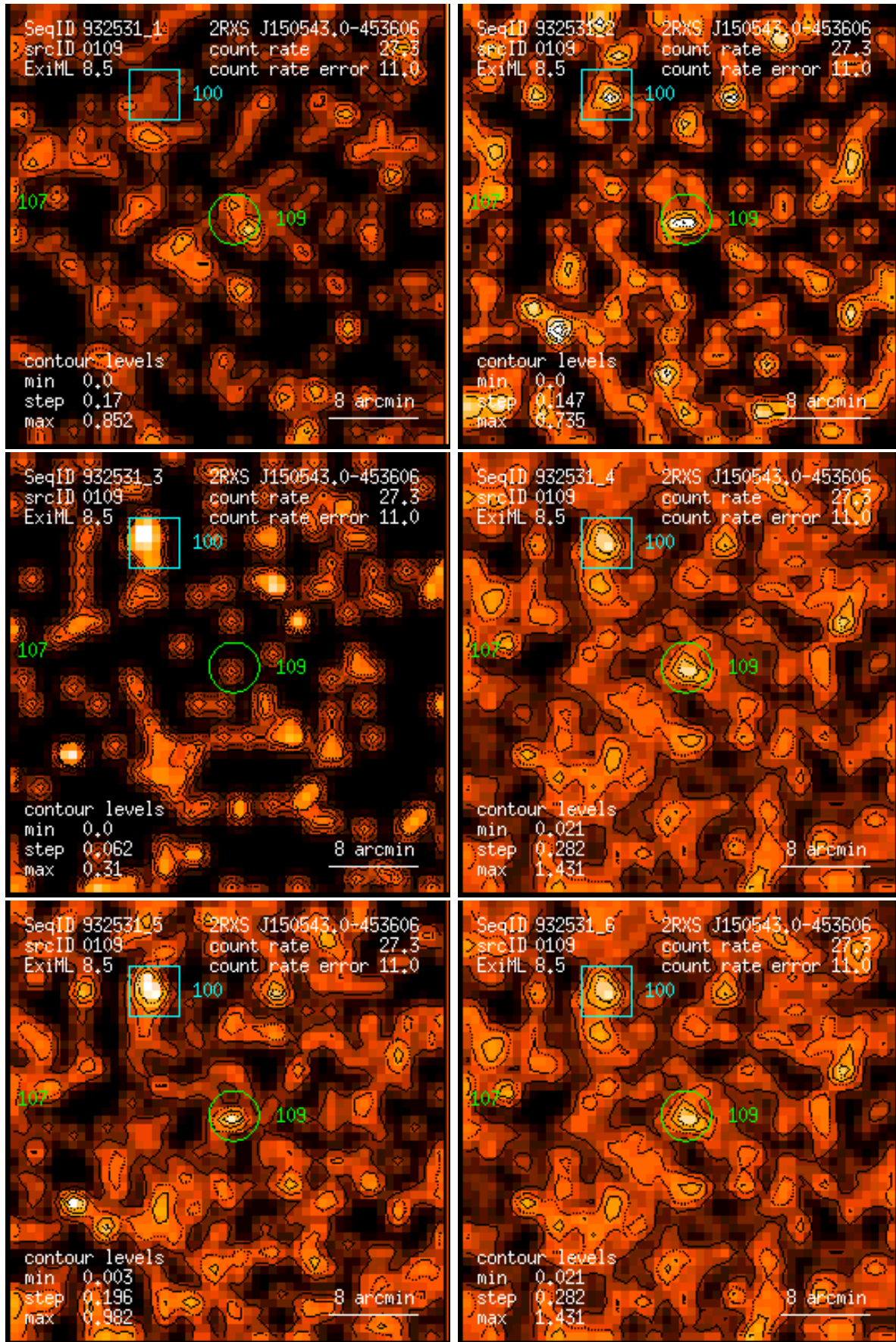
Figure 109: RASS 932531: detection 0109: band rate images, Gaussian filter: (1) PSPC channels 11 – 41, (2) 52 – 90, (3) 91 – 201, (4) 11 – 235, (5) 52 – 201, (6) 11 – 201. Broad band rates in counts/ks. Band rate contour levels in counts/ks/arcmin 2 .
