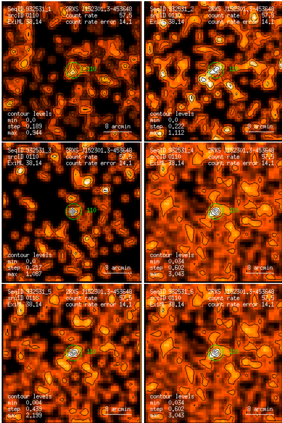
Figure 110: RASS 932531: detection 0110: band rate images, Gaussian filter: (1) PSPC channels 11 – 41, (2) 52 – 90, (3) 91 – 201, (4) 11 – 235, (5) 52 – 201, (6) 11 – 201. Broad band rates in counts/ks. Band rate contour levels in counts/ks/arcmin 2 .
