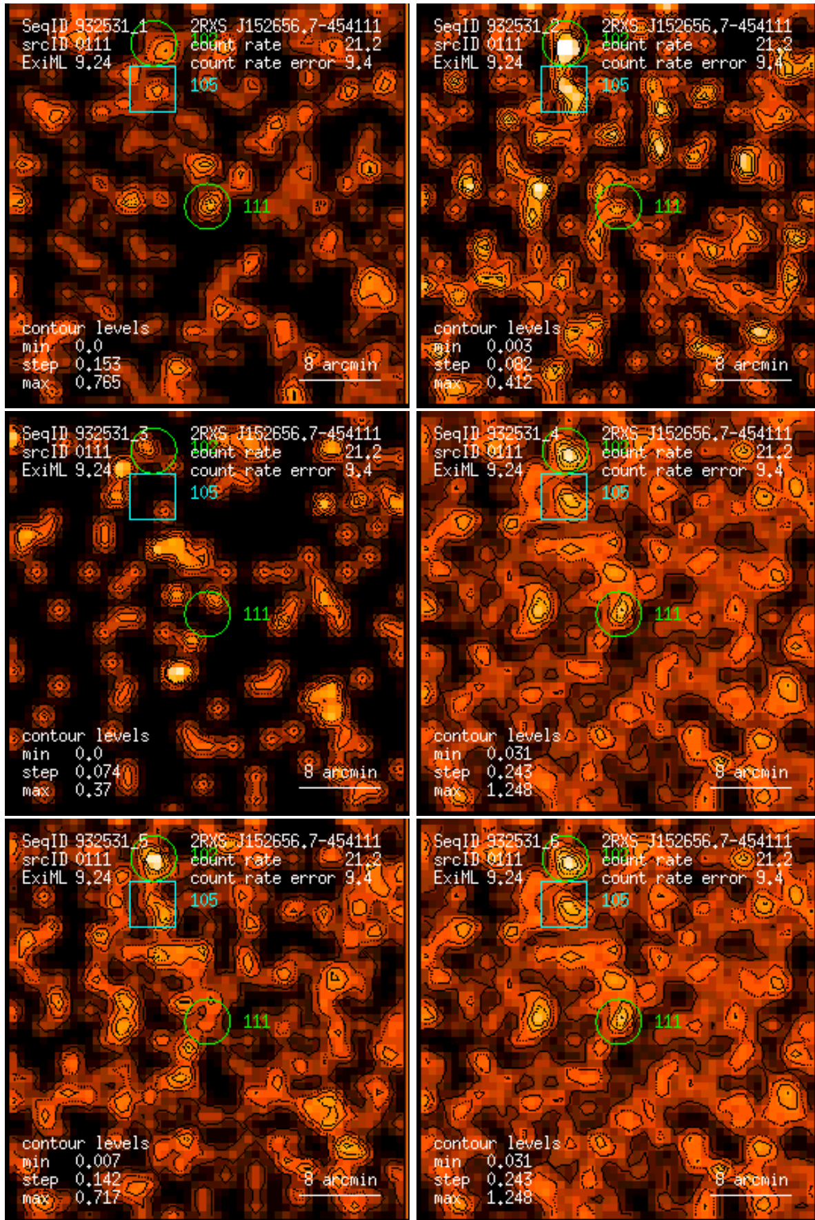
Figure 111: RASS 932531: detection 0111: band rate images, Gaussian filter: (1) PSPC channels 11 – 41, (2) 52 – 90, (3) 91 – 201, (4) 11 – 235, (5) 52 – 201, (6) 11 – 201. Broad band rates in counts/ks. Band rate contour levels in counts/ks/arcmin 2 .
