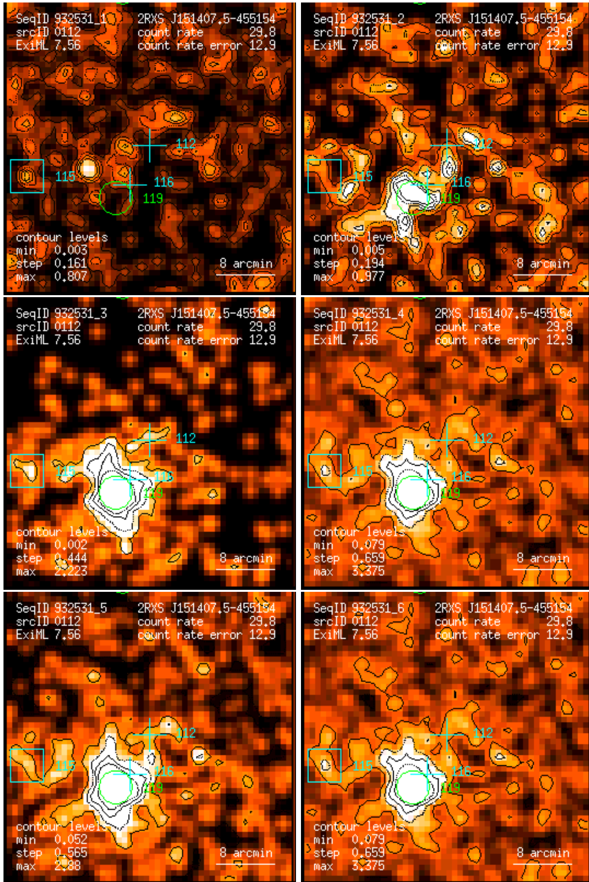
Figure 112: RASS 932531: detection 0112: band rate images, Gaussian filter: (1) PSPC channels 11 – 41, (2) 52 – 90, (3) 91 – 201, (4) 11 – 235, (5) 52 – 201, (6) 11 – 201. Broad band rates in counts/ks. Band rate contour levels in counts/ks/arcmin 2 .
