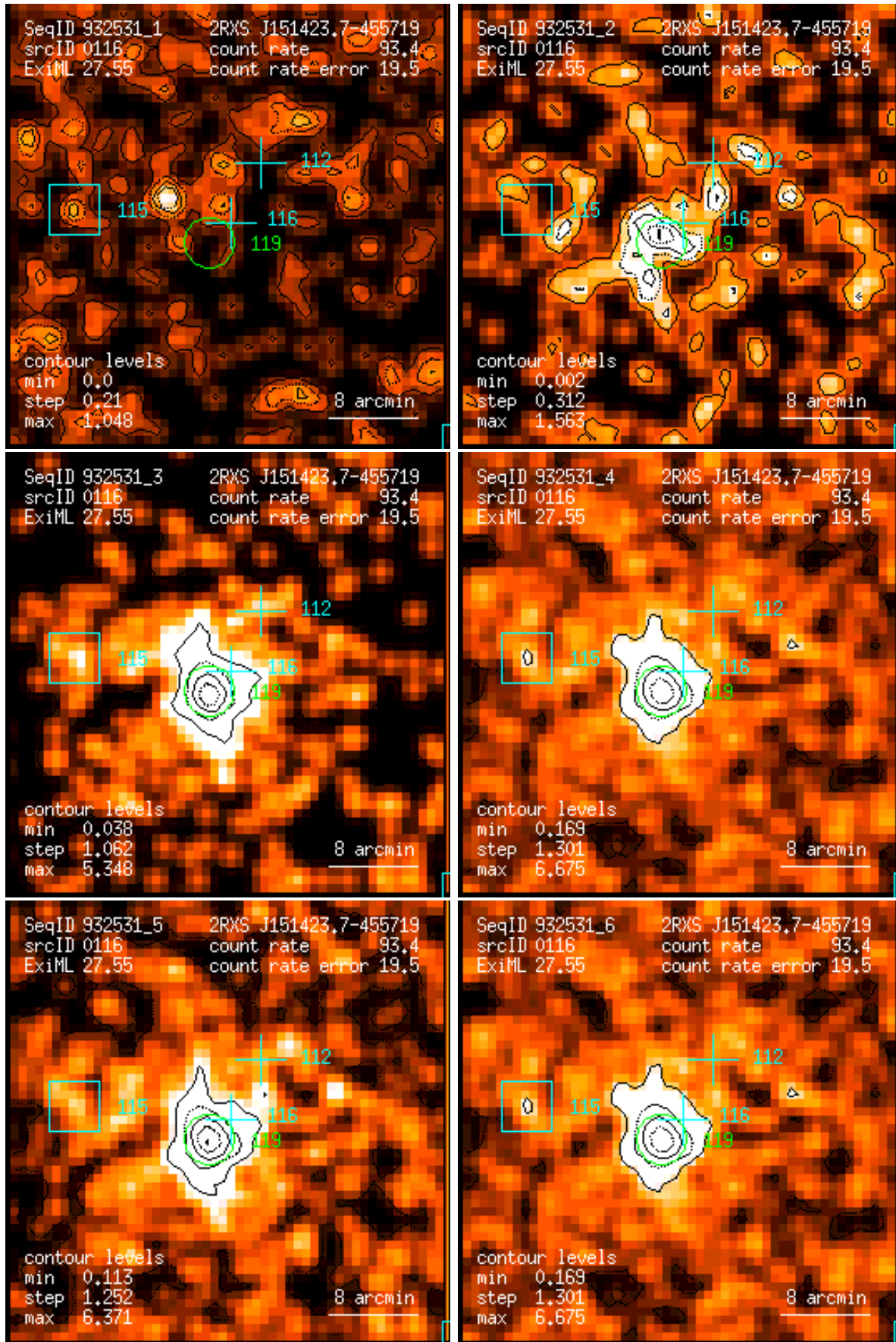
Figure 116: RASS 932531: detection 0116: band rate images, Gaussian filter: (1) PSPC channels 11 – 41, (2) 52 – 90, (3) 91 – 201, (4) 11 – 235, (5) 52 – 201, (6) 11 – 201. Broad band rates in counts/ks. Band rate contour levels in counts/ks/arcmin 2 .
