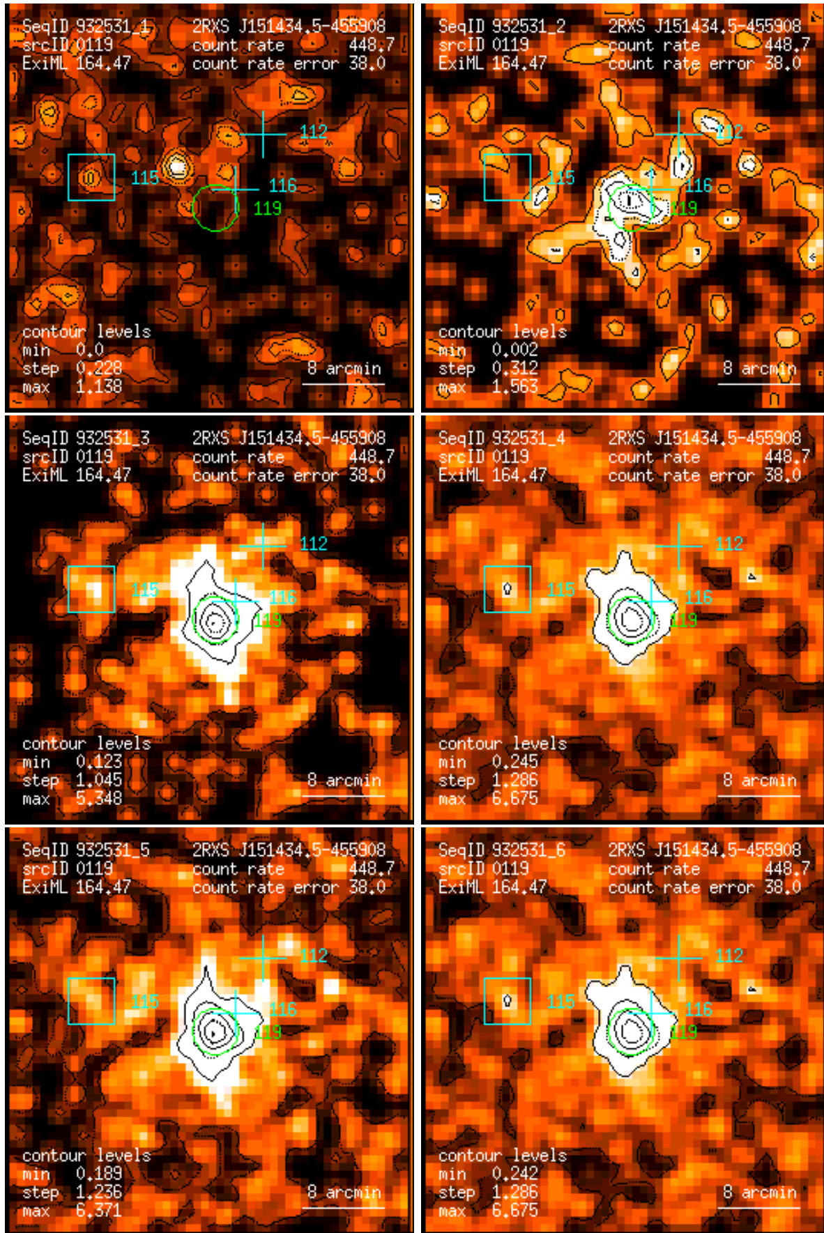
Figure 119: RASS 932531: detection 0119: band rate images, Gaussian filter: (1) PSPC channels 11 – 41, (2) 52 – 90, (3) 91 – 201, (4) 11 – 235, (5) 52 – 201, (6) 11 – 201. Broad band rates in counts/ks. Band rate contour levels in counts/ks/arcmin 2 .
