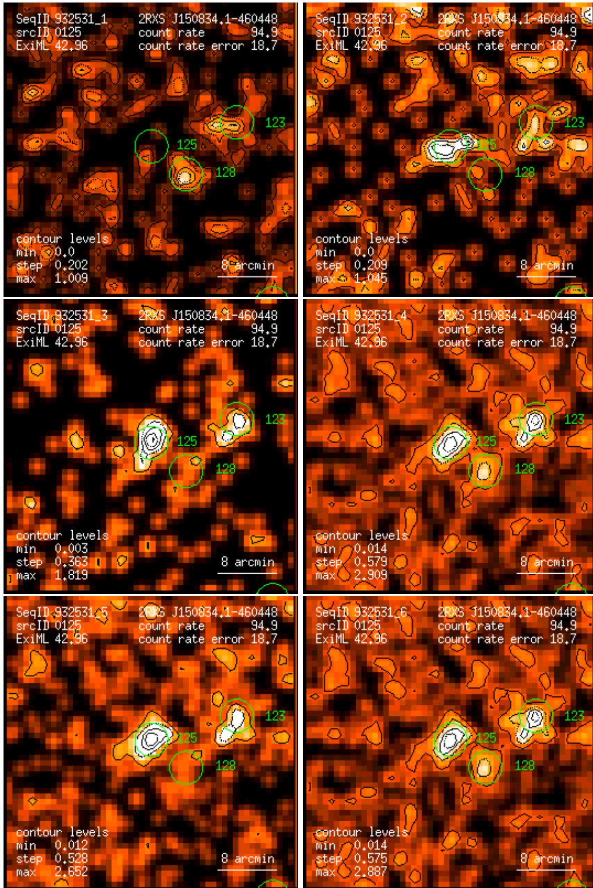
Figure 125: RASS 932531: detection 0125: band rate images, Gaussian filter: (1) PSPC channels 11 – 41, (2) 52 – 90, (3) 91 – 201, (4) 11 – 235, (5) 52 – 201, (6) 11 – 201. Broad band rates in counts/ks. Band rate contour levels in counts/ks/arcmin 2 .
