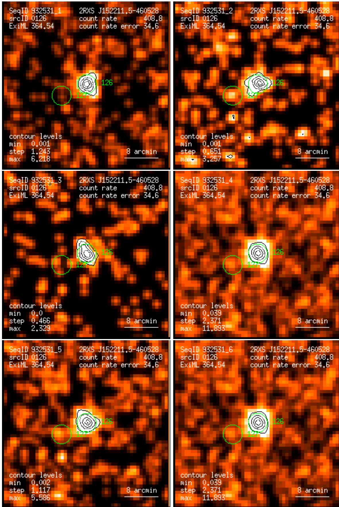
Figure 126: RASS 932531: detection 0126: band rate images, Gaussian filter: (1) PSPC channels 11 – 41, (2) 52 – 90, (3) 91 – 201, (4) 11 – 235, (5) 52 – 201, (6) 11 – 201. Broad band rates in counts/ks. Band rate contour levels in counts/ks/arcmin 2 .
