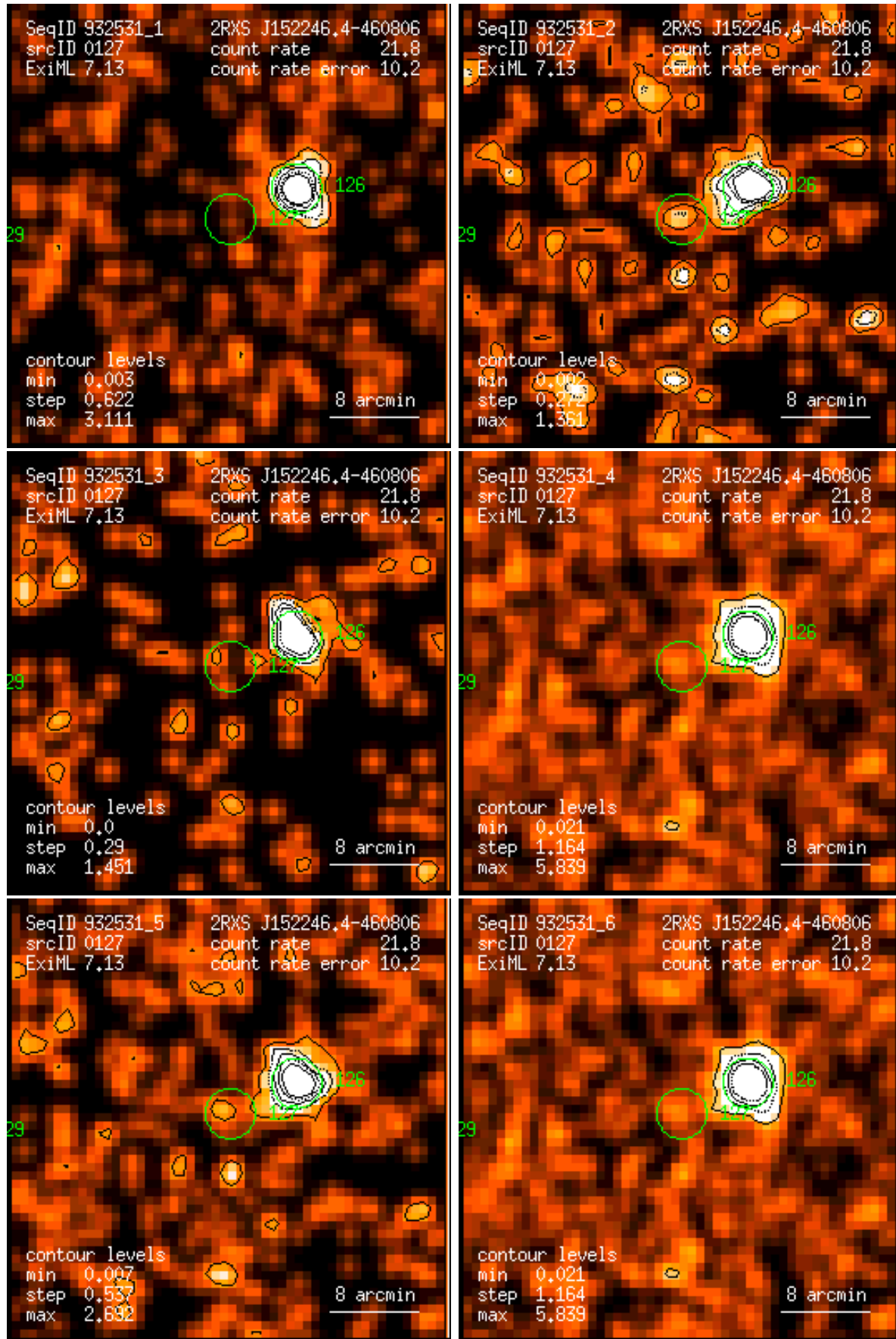
Figure 127: RASS 932531: detection 0127: band rate images, Gaussian filter: (1) PSPC channels 11 – 41, (2) 52 – 90, (3) 91 – 201, (4) 11 – 235, (5) 52 – 201, (6) 11 – 201. Broad band rates in counts/ks. Band rate contour levels in counts/ks/arcmin 2 .
