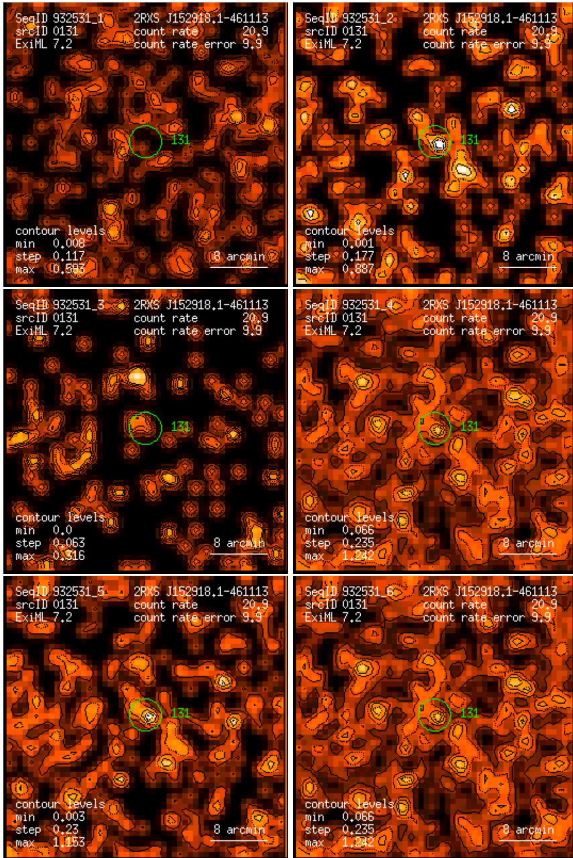
Figure 131: RASS 932531: detection 0131: band rate images, Gaussian filter: (1) PSPC channels 11 – 41, (2) 52 – 90, (3) 91 – 201, (4) 11 – 235, (5) 52 – 201, (6) 11 – 201. Broad band rates in counts/ks. Band rate contour levels in counts/ks/arcmin 2 .
