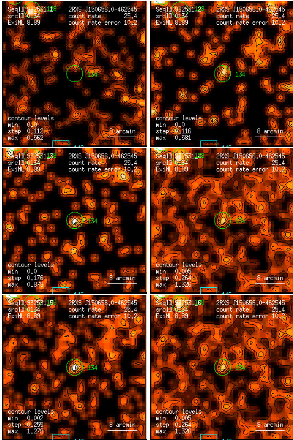
Figure 134: RASS 932531: detection 0134: band rate images, Gaussian filter: (1) PSPC channels 11 – 41, (2) 52 – 90, (3) 91 – 201, (4) 11 – 235, (5) 52 – 201, (6) 11 – 201. Broad band rates in counts/ks. Band rate contour levels in counts/ks/arcmin 2 .
