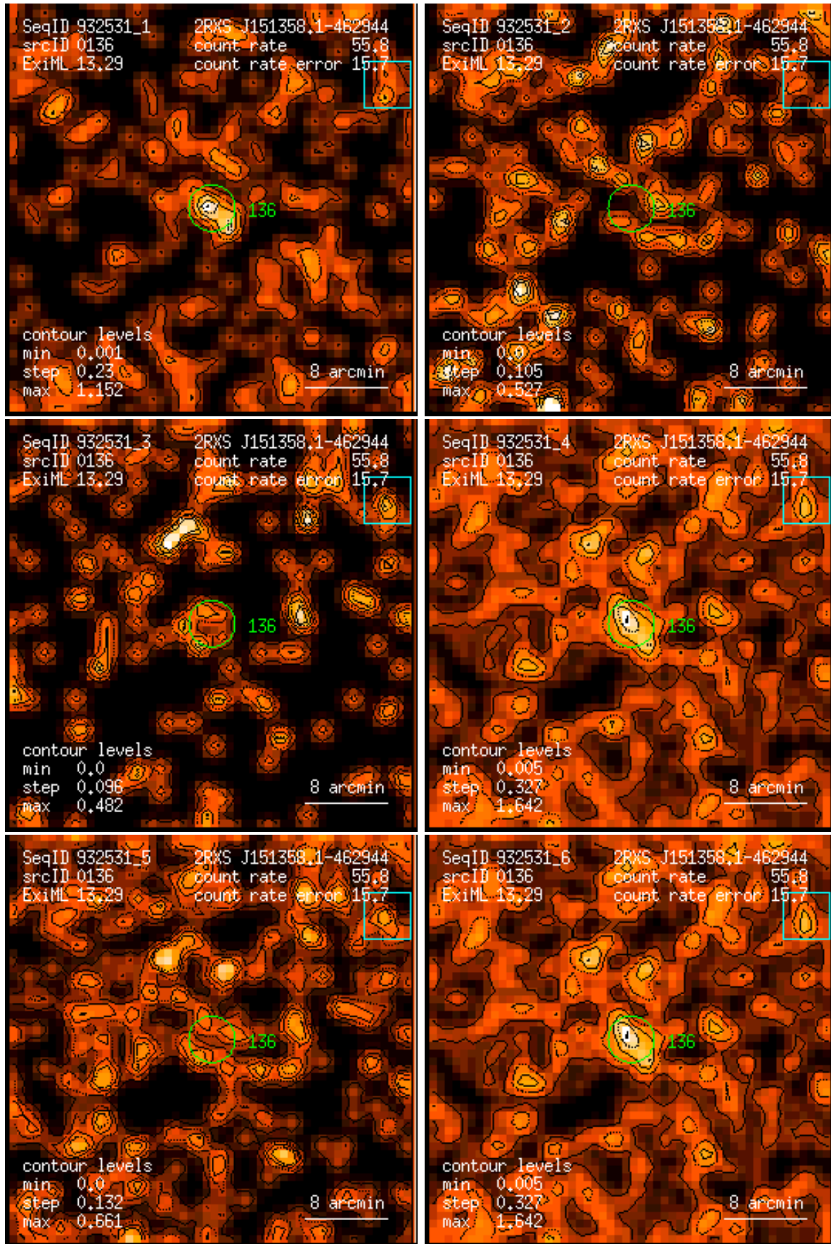
Figure 136: RASS 932531: detection 0136: band rate images, Gaussian filter: (1) PSPC channels 11 – 41, (2) 52 – 90, (3) 91 – 201, (4) 11 – 235, (5) 52 – 201, (6) 11 – 201. Broad band rates in counts/ks. Band rate contour levels in counts/ks/arcmin 2 .
