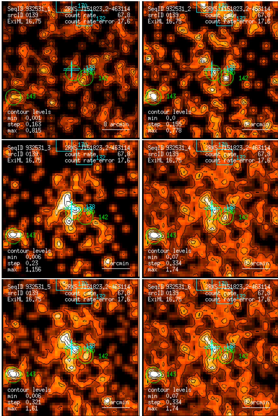
Figure 139: RASS 932531: detection 0139: band rate images, Gaussian filter: (1) PSPC channels 11 – 41, (2) 52 – 90, (3) 91 – 201, (4) 11 – 235, (5) 52 – 201, (6) 11 – 201. Broad band rates in counts/ks. Band rate contour levels in counts/ks/arcmin 2 .
