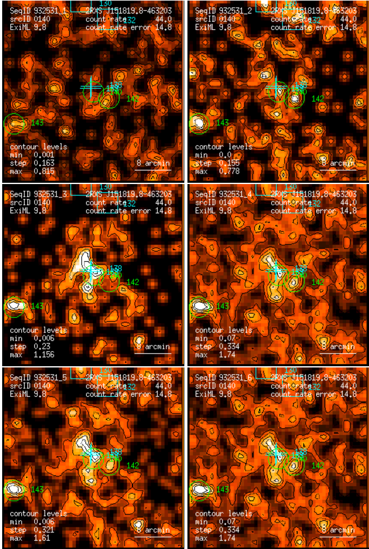
Figure 140: RASS 932531: detection 0140: band rate images, Gaussian filter: (1) PSPC channels 11 – 41, (2) 52 – 90, (3) 91 – 201, (4) 11 – 235, (5) 52 – 201, (6) 11 – 201. Broad band rates in counts/ks. Band rate contour levels in counts/ks/arcmin 2 .
