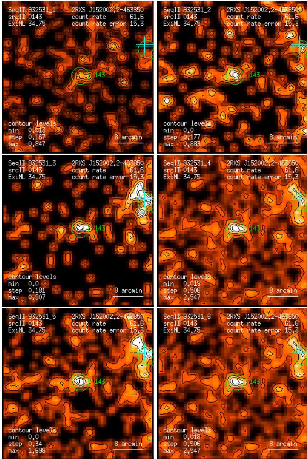
Figure 143: RASS 932531: detection 0143: band rate images, Gaussian filter: (1) PSPC channels 11 – 41, (2) 52 – 90, (3) 91 – 201, (4) 11 – 235, (5) 52 – 201, (6) 11 – 201. Broad band rates in counts/ks. Band rate contour levels in counts/ks/arcmin 2 .
