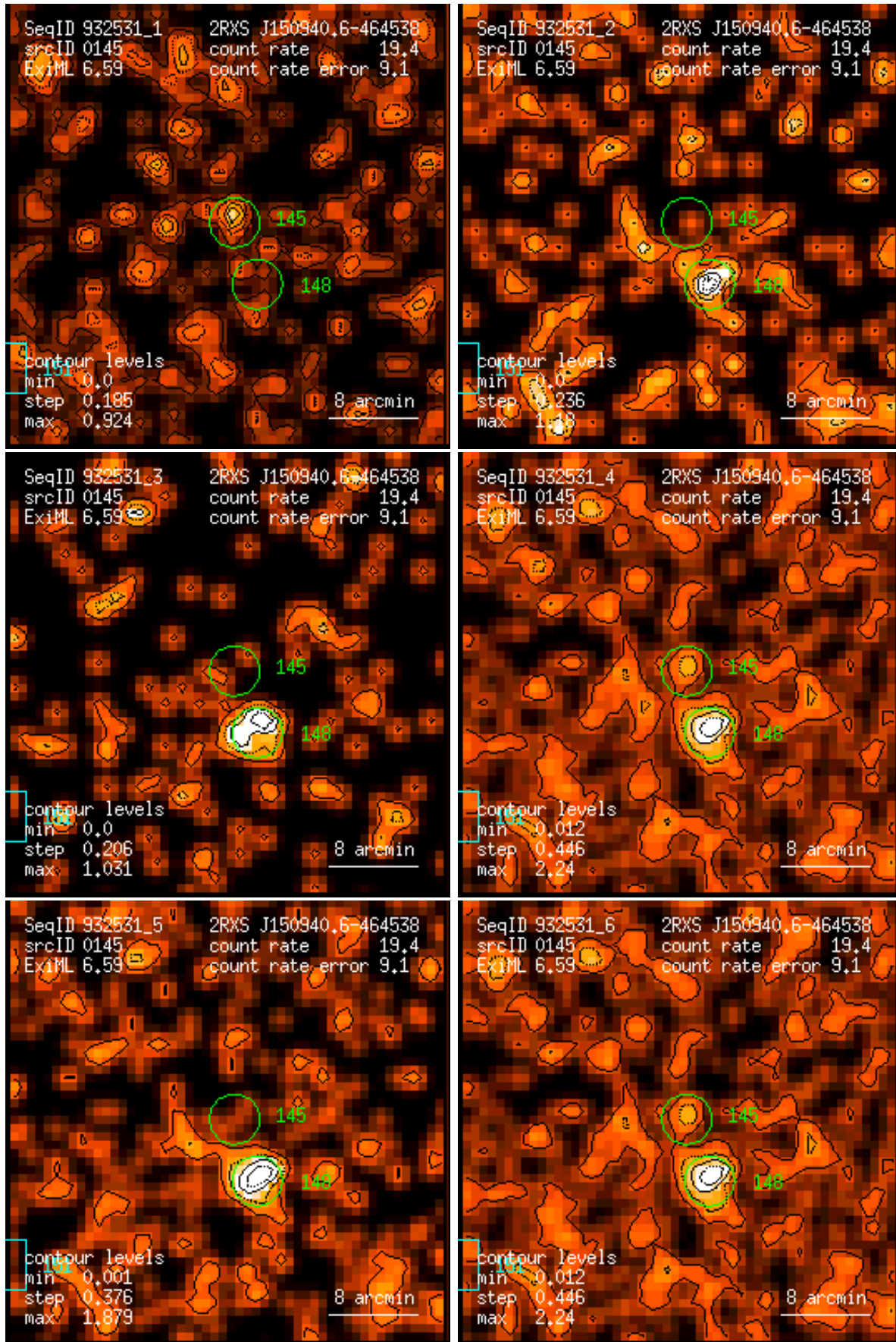
Figure 145: RASS 932531: detection 0145: band rate images, Gaussian filter: (1) PSPC channels 11 – 41, (2) 52 – 90, (3) 91 – 201, (4) 11 – 235, (5) 52 – 201, (6) 11 – 201. Broad band rates in counts/ks. Band rate contour levels in counts/ks/arcmin 2 .
