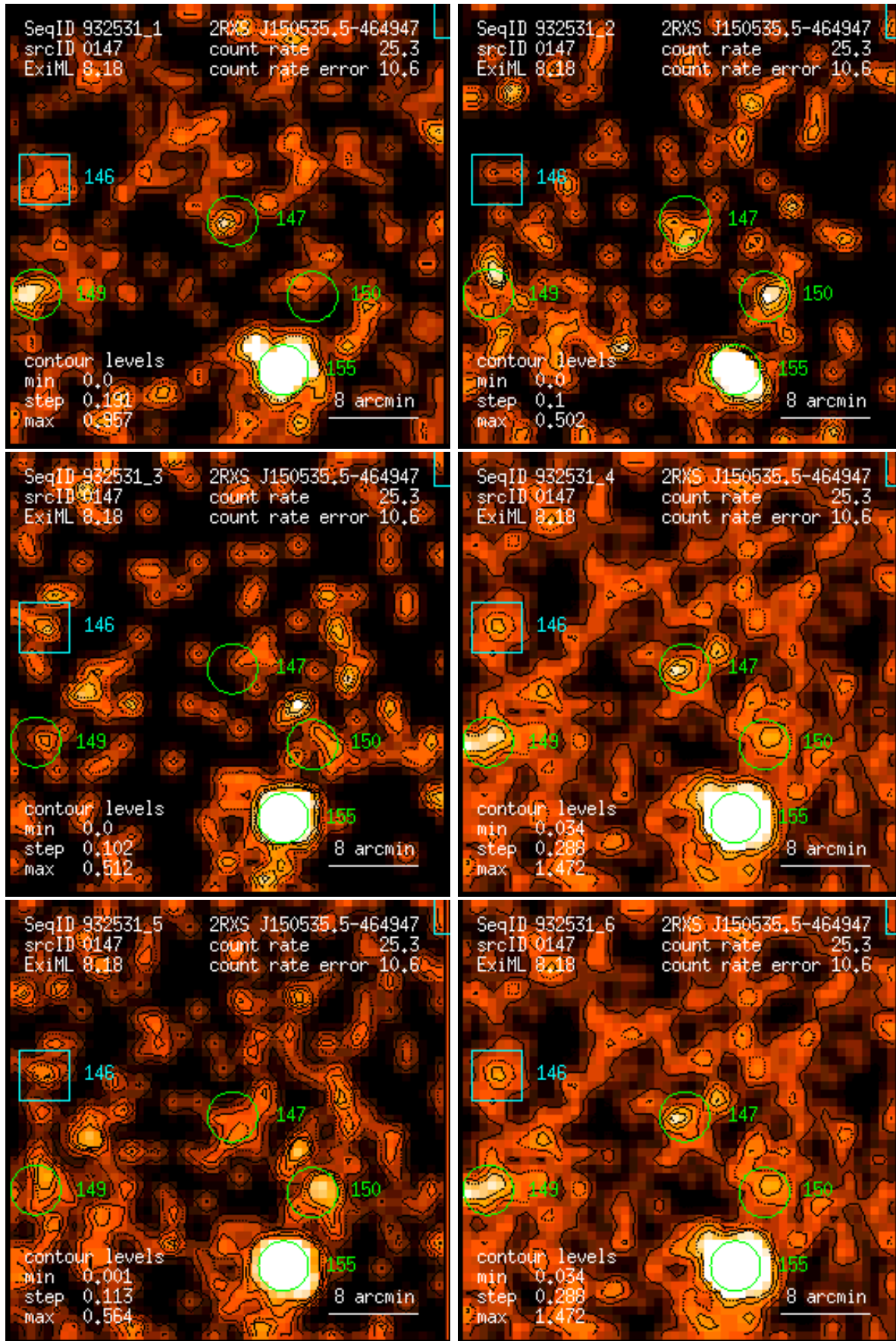
Figure 147: RASS 932531: detection 0147: band rate images, Gaussian filter: (1) PSPC channels 11 – 41, (2) 52 – 90, (3) 91 – 201, (4) 11 – 235, (5) 52 – 201, (6) 11 – 201. Broad band rates in counts/ks. Band rate contour levels in counts/ks/arcmin 2 .
