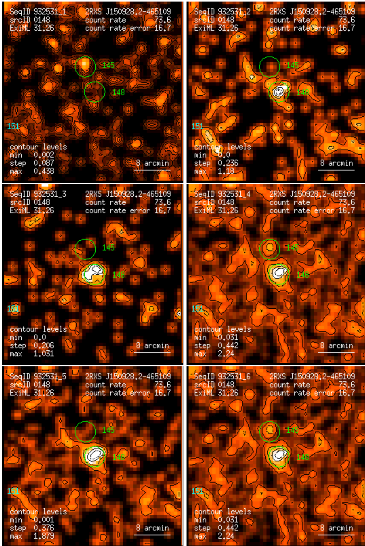
Figure 148: RASS 932531: detection 0148: band rate images, Gaussian filter: (1) PSPC channels 11 – 41, (2) 52 – 90, (3) 91 – 201, (4) 11 – 235, (5) 52 – 201, (6) 11 – 201. Broad band rates in counts/ks. Band rate contour levels in counts/ks/arcmin 2 .
