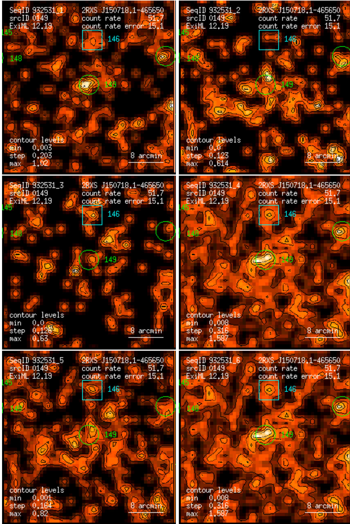
Figure 149: RASS 932531: detection 0149: band rate images, Gaussian filter: (1) PSPC channels 11 – 41, (2) 52 – 90, (3) 91 – 201, (4) 11 – 235, (5) 52 – 201, (6) 11 – 201. Broad band rates in counts/ks. Band rate contour levels in counts/ks/arcmin 2 .
