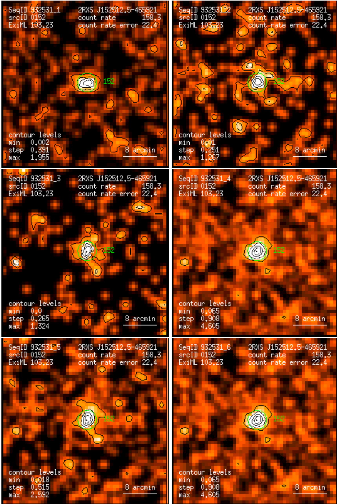
Figure 152: RASS 932531: detection 0152: band rate images, Gaussian filter: (1) PSPC channels 11 – 41, (2) 52 – 90, (3) 91 – 201, (4) 11 – 235, (5) 52 – 201, (6) 11 – 201. Broad band rates in counts/ks. Band rate contour levels in counts/ks/arcmin 2 .
