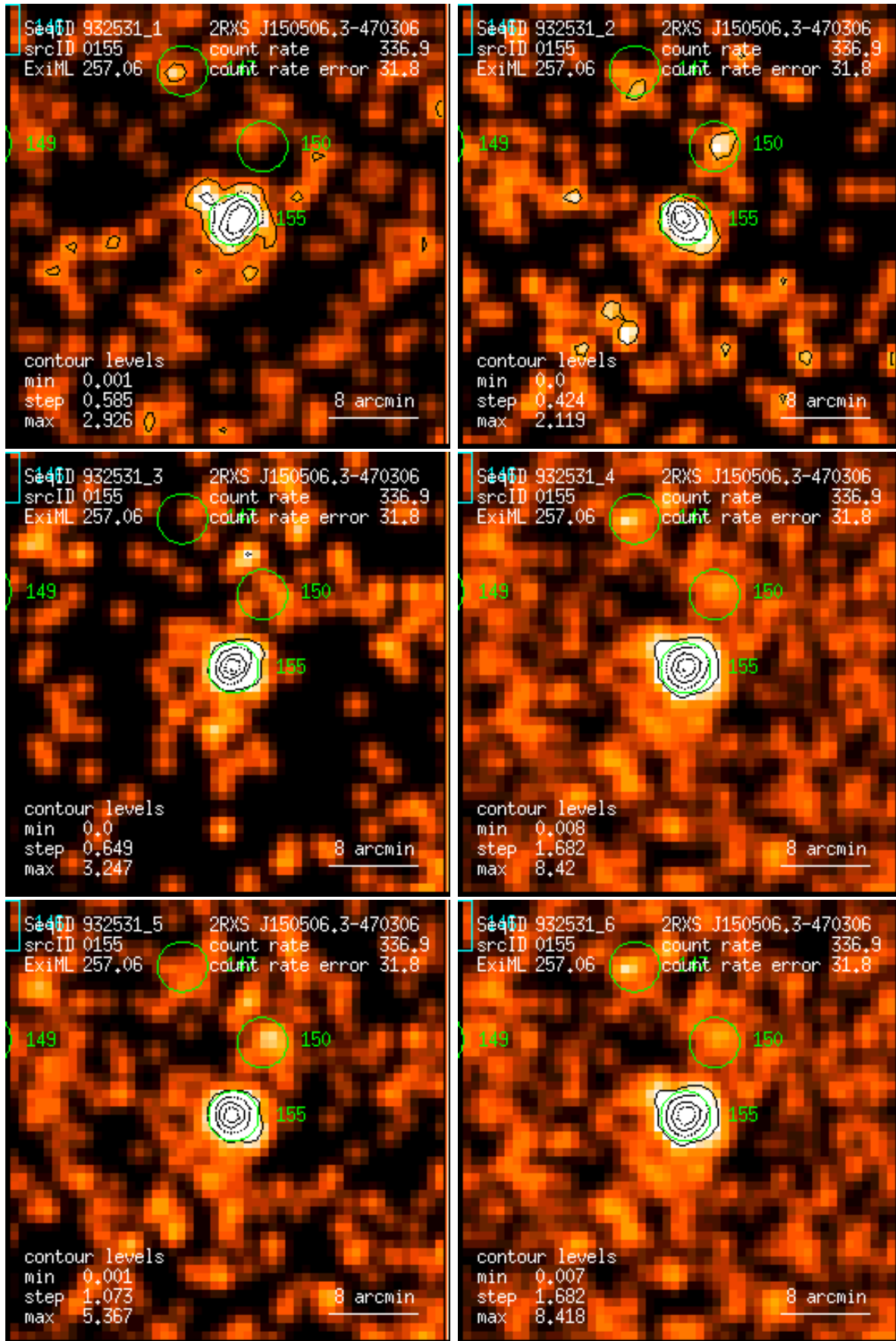
Figure 155: RASS 932531: detection 0155: band rate images, Gaussian filter: (1) PSPC channels 11 – 41, (2) 52 – 90, (3) 91 – 201, (4) 11 – 235, (5) 52 – 201, (6) 11 – 201. Broad band rates in counts/ks. Band rate contour levels in counts/ks/arcmin 2 .
