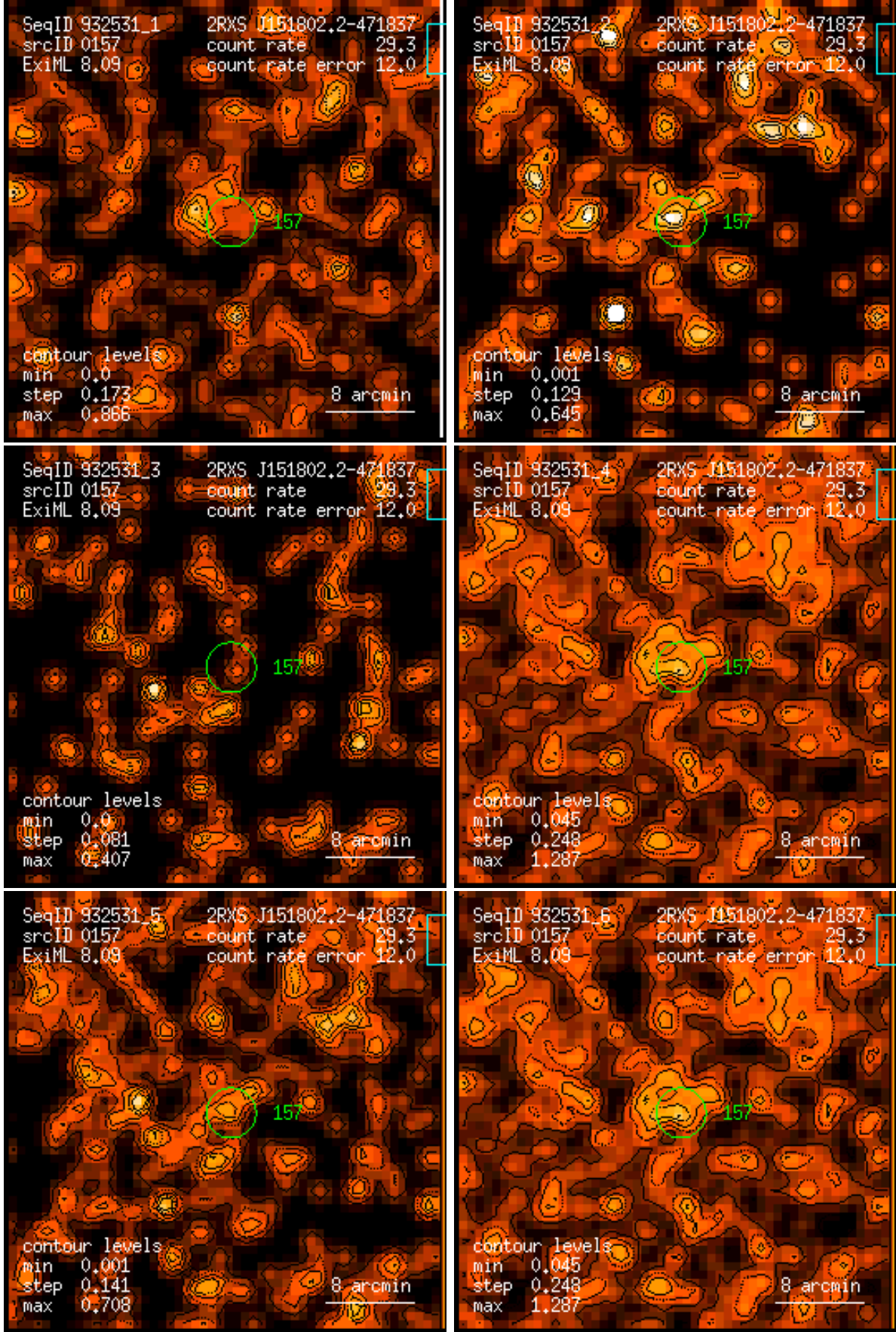
Figure 157: RASS 932531: detection 0157: band rate images, Gaussian filter: (1) PSPC channels 11 – 41, (2) 52 – 90, (3) 91 – 201, (4) 11 – 235, (5) 52 – 201, (6) 11 – 201. Broad band rates in counts/ks. Band rate contour levels in counts/ks/arcmin 2 .
