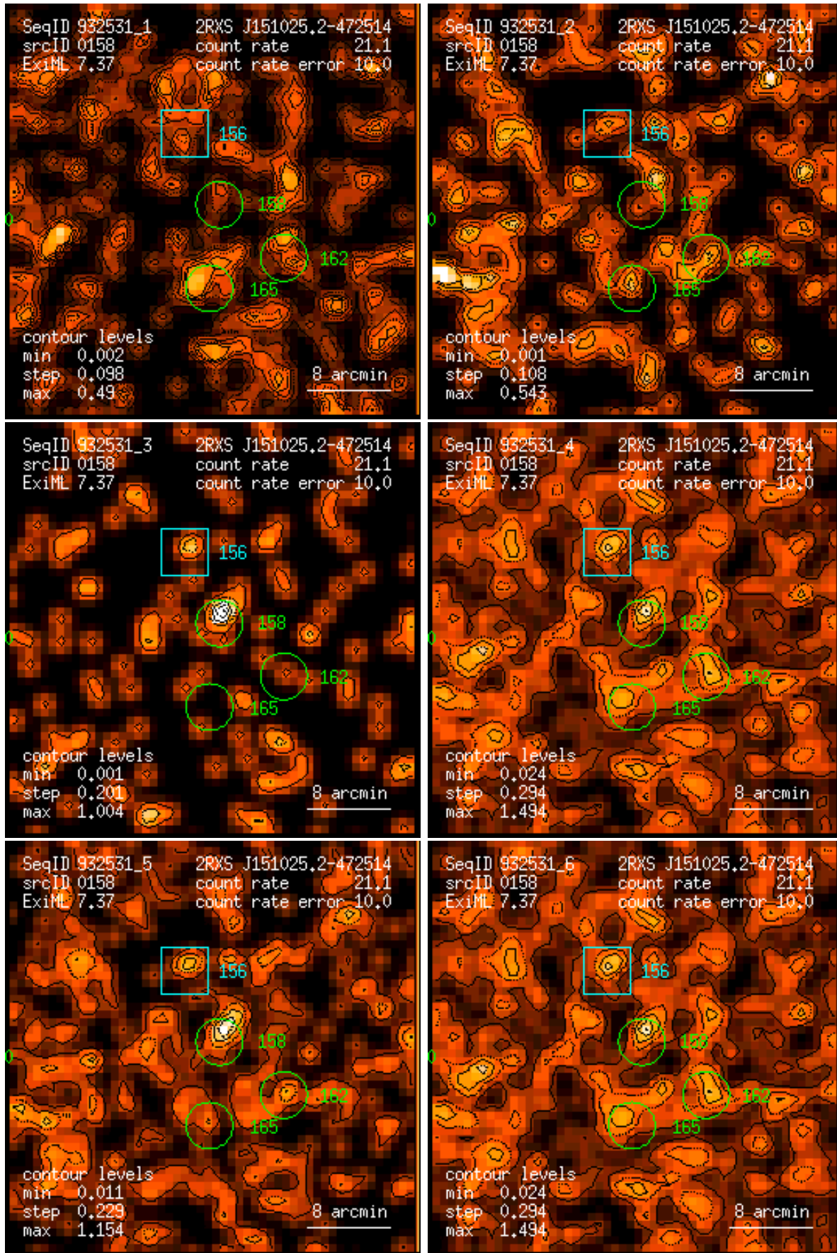
Figure 158: RASS 932531: detection 0158: band rate images, Gaussian filter: (1) PSPC channels 11 – 41, (2) 52 – 90, (3) 91 – 201, (4) 11 – 235, (5) 52 – 201, (6) 11 – 201. Broad band rates in counts/ks. Band rate contour levels in counts/ks/arcmin 2 .
