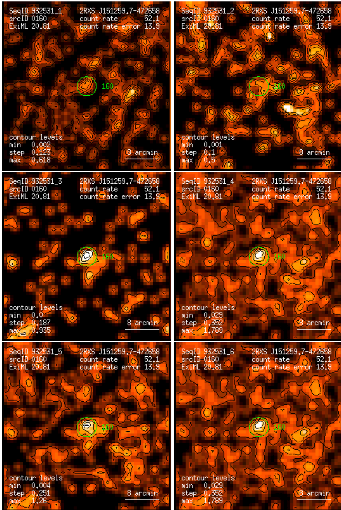
Figure 160: RASS 932531: detection 0160: band rate images, Gaussian filter: (1) PSPC channels 11 – 41, (2) 52 – 90, (3) 91 – 201, (4) 11 – 235, (5) 52 – 201, (6) 11 – 201. Broad band rates in counts/ks. Band rate contour levels in counts/ks/arcmin 2 .
