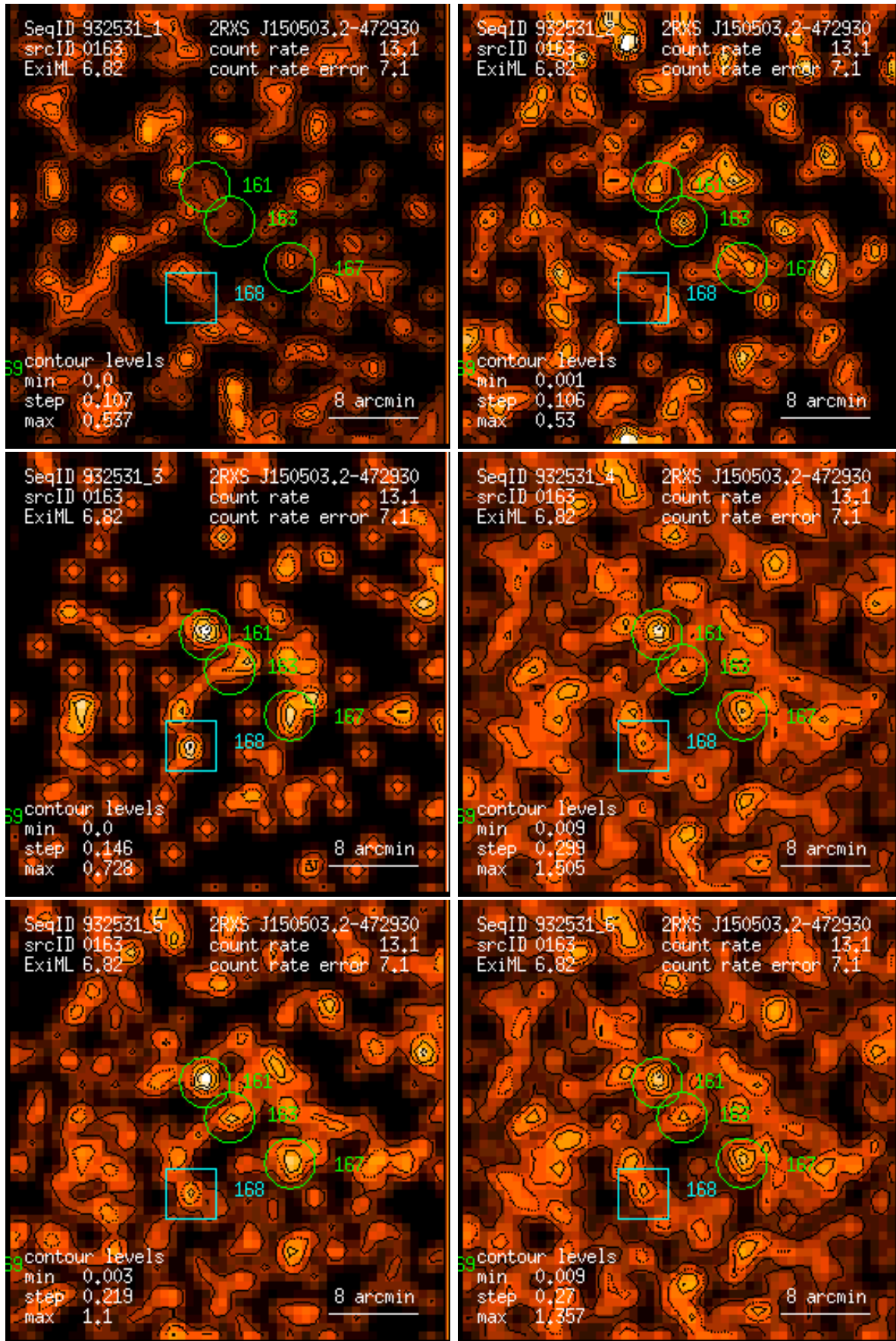
Figure 163: RASS 932531: detection 0163: band rate images, Gaussian filter: (1) PSPC channels 11 – 41, (2) 52 – 90, (3) 91 – 201, (4) 11 – 235, (5) 52 – 201, (6) 11 – 201. Broad band rates in counts/ks. Band rate contour levels in counts/ks/arcmin 2 .
