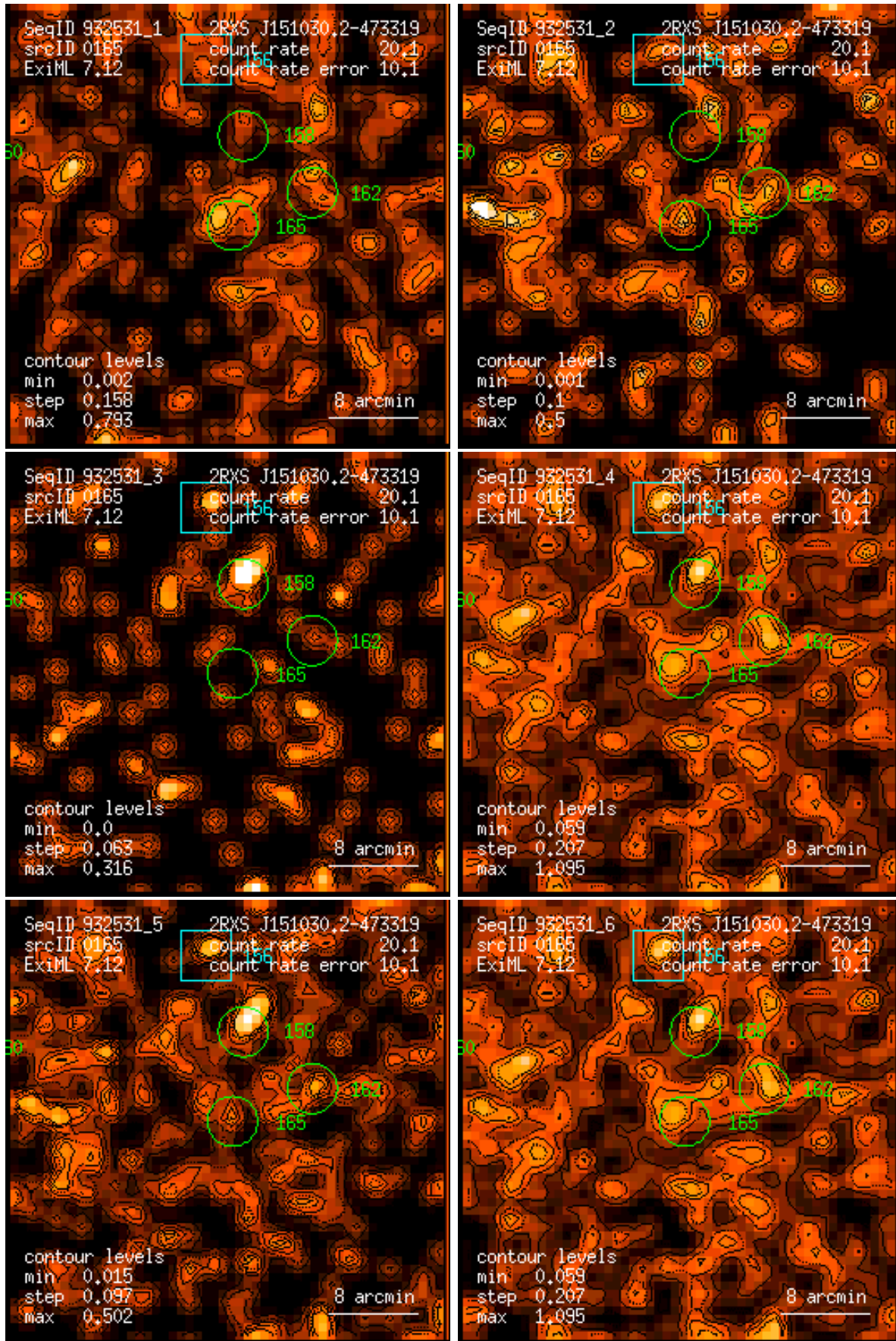
Figure 165: RASS 932531: detection 0165: band rate images, Gaussian filter: (1) PSPC channels 11 – 41, (2) 52 – 90, (3) 91 – 201, (4) 11 – 235, (5) 52 – 201, (6) 11 – 201. Broad band rates in counts/ks. Band rate contour levels in counts/ks/arcmin 2 .
