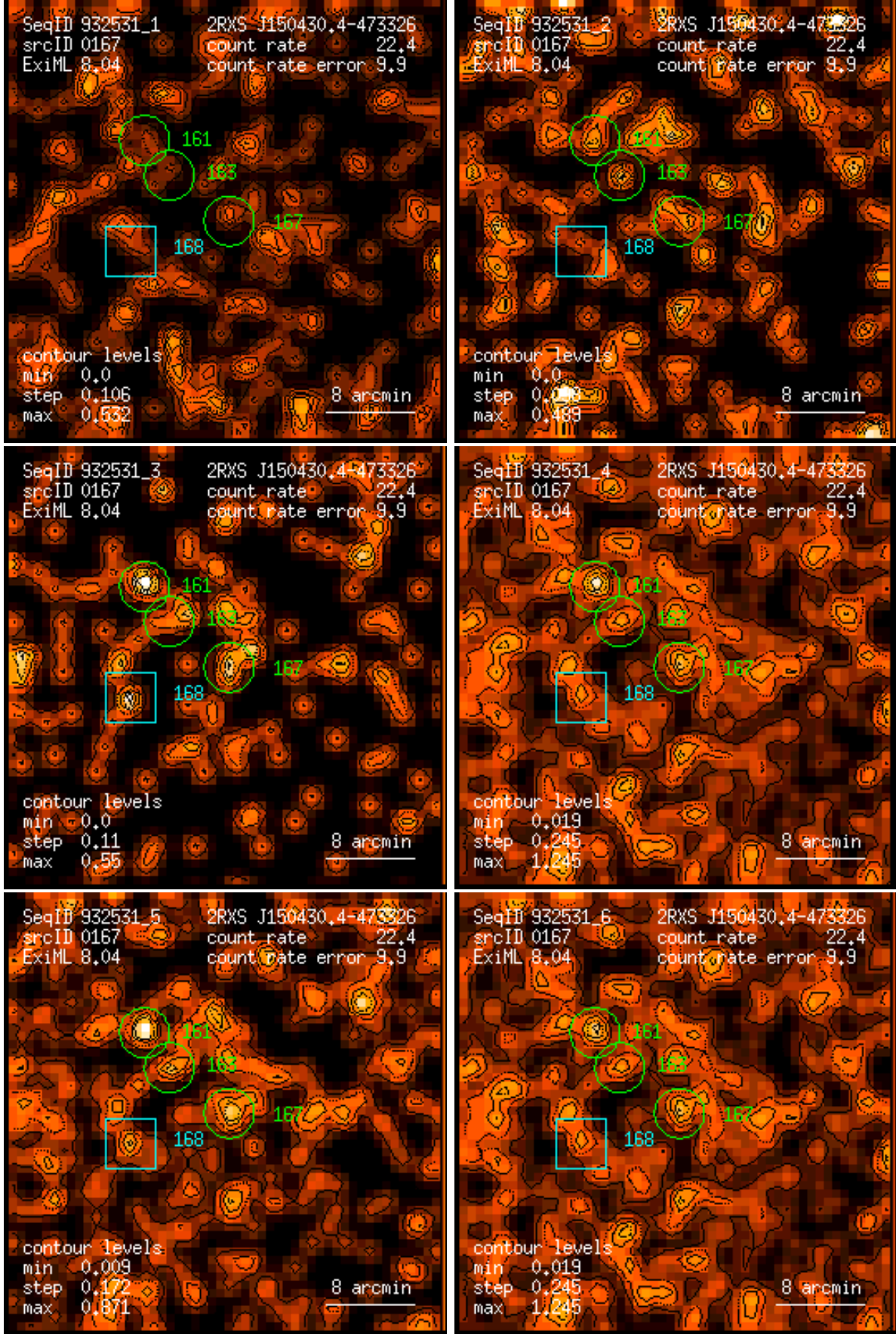
Figure 167: RASS 932531: detection 0167: band rate images, Gaussian filter: (1) PSPC channels 11 – 41, (2) 52 – 90, (3) 91 – 201, (4) 11 – 235, (5) 52 – 201, (6) 11 – 201. Broad band rates in counts/ks. Band rate contour levels in counts/ks/arcmin 2 .
