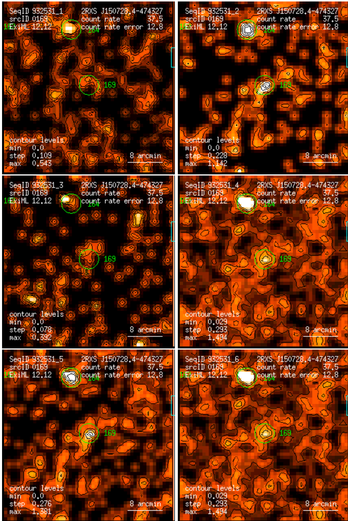
Figure 169: RASS 932531: detection 0169: band rate images, Gaussian filter: (1) PSPC channels 11 – 41, (2) 52 – 90, (3) 91 – 201, (4) 11 – 235, (5) 52 – 201, (6) 11 – 201. Broad band rates in counts/ks. Band rate contour levels in counts/ks/arcmin 2 .
