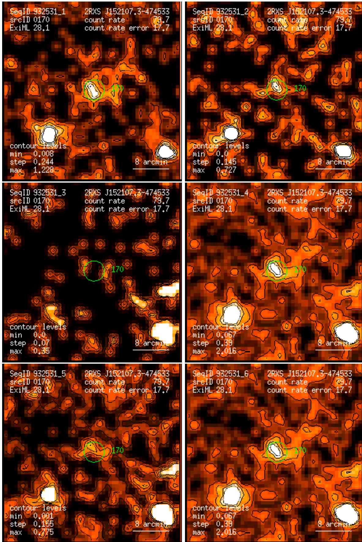
Figure 170: RASS 932531: detection 0170: band rate images, Gaussian filter: (1) PSPC channels 11 – 41, (2) 52 – 90, (3) 91 – 201, (4) 11 – 235, (5) 52 – 201, (6) 11 – 201. Broad band rates in counts/ks. Band rate contour levels in counts/ks/arcmin 2 .
