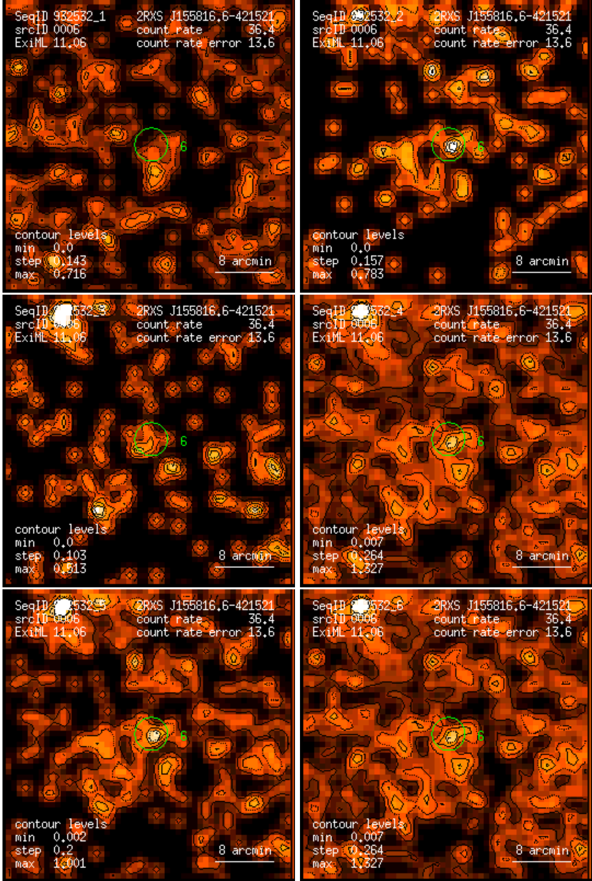
Figure 6: RASS 932532: detection 0006: band rate images, Gaussian filter: (1) PSPC channels 11 – 41, (2) 52 – 90, (3) 91 – 201, (4) 11 – 235, (5) 52 – 201, (6) 11 – 201. Broad band rates in counts/ks. Band rate contour levels in counts/ks/arcmin 2 .
