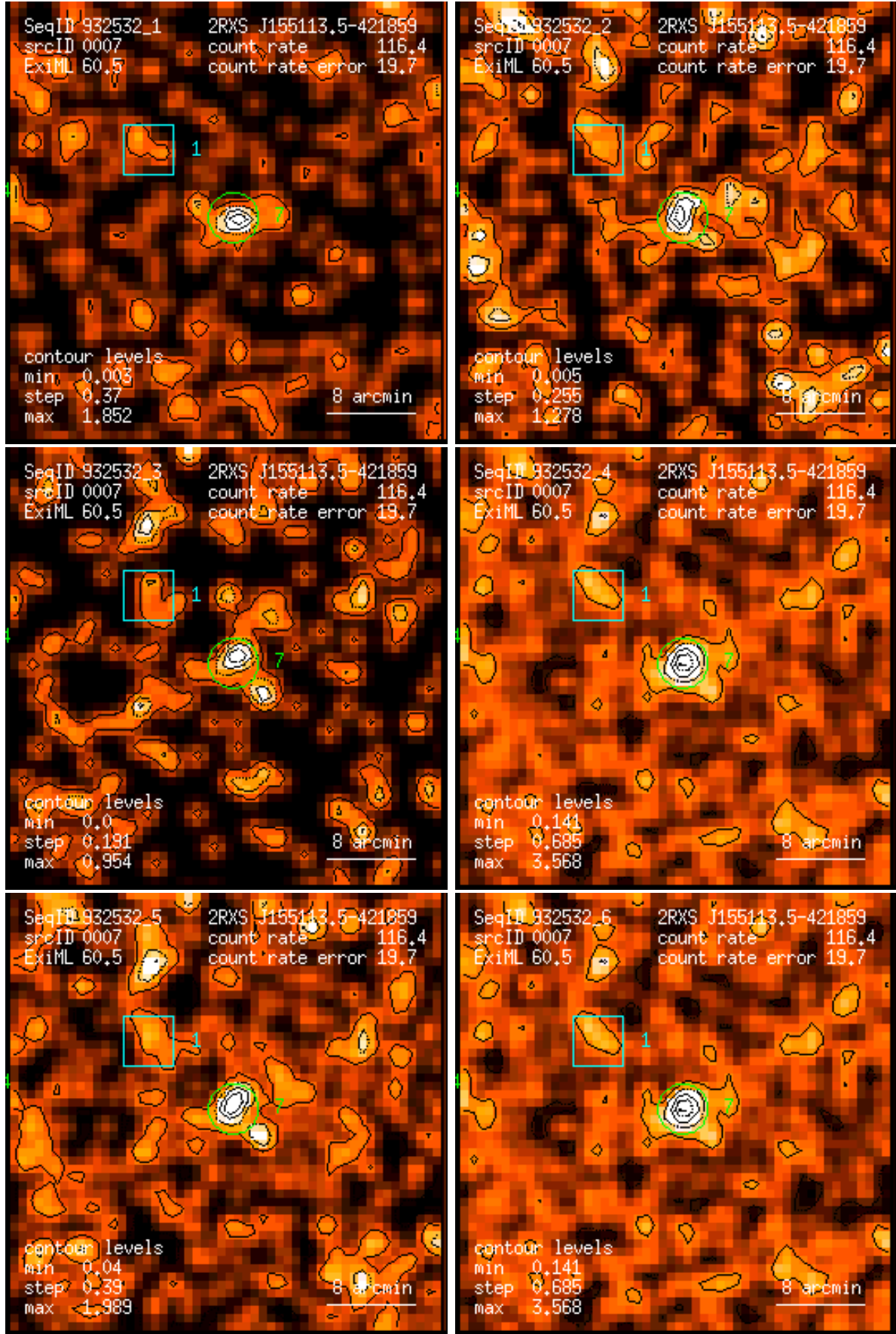
Figure 7: RASS 932532: detection 0007: band rate images, Gaussian filter: (1) PSPC channels 11 – 41, (2) 52 – 90, (3) 91 – 201, (4) 11 – 235, (5) 52 – 201, (6) 11 – 201. Broad band rates in counts/ks. Band rate contour levels in counts/ks/arcmin 2 .
