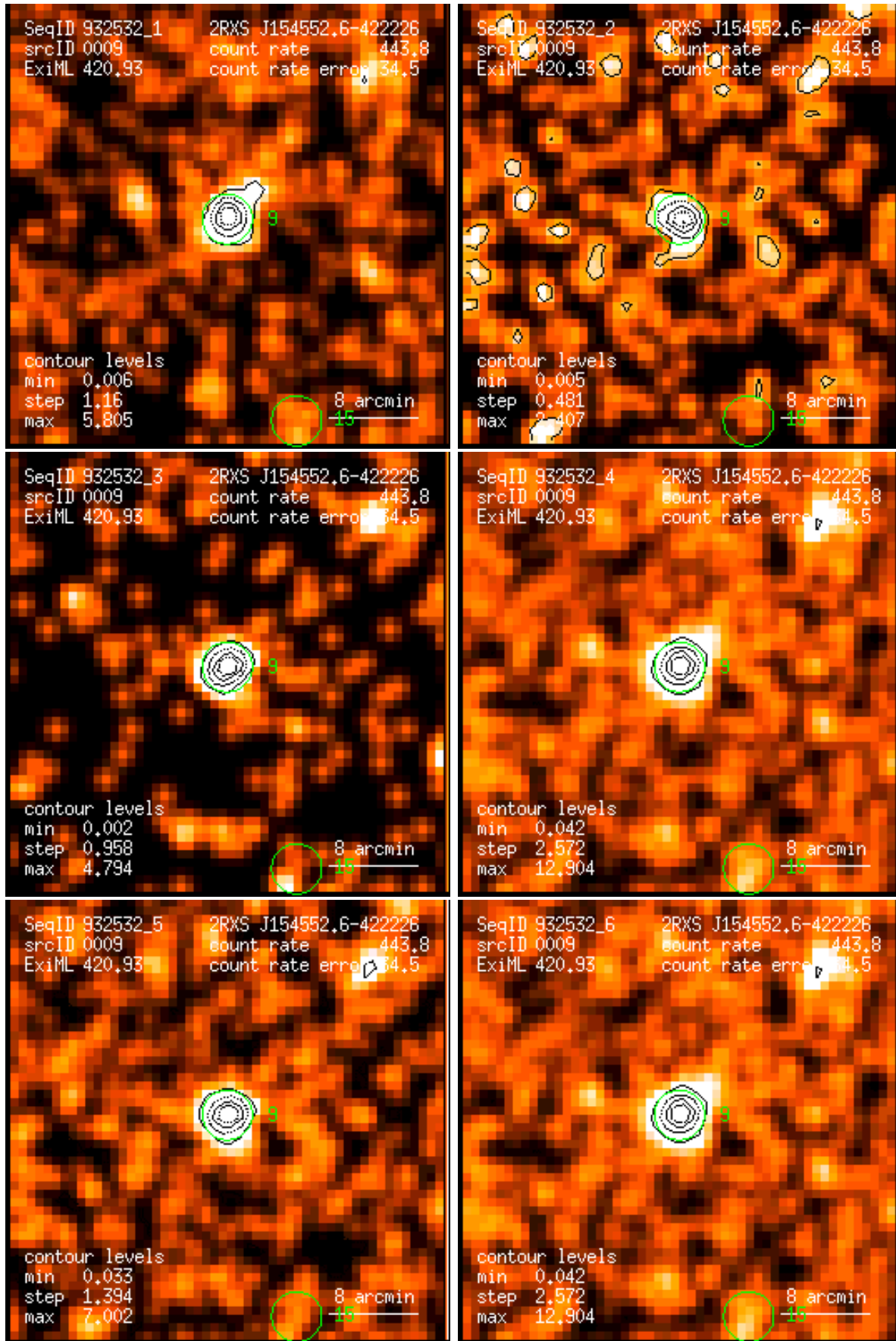
Figure 9: RASS 932532: detection 0009: band rate images, Gaussian filter: (1) PSPC channels 11 – 41, (2) 52 – 90, (3) 91 – 201, (4) 11 – 235, (5) 52 – 201, (6) 11 – 201. Broad band rates in counts/ks. Band rate contour levels in counts/ks/arcmin 2 .
