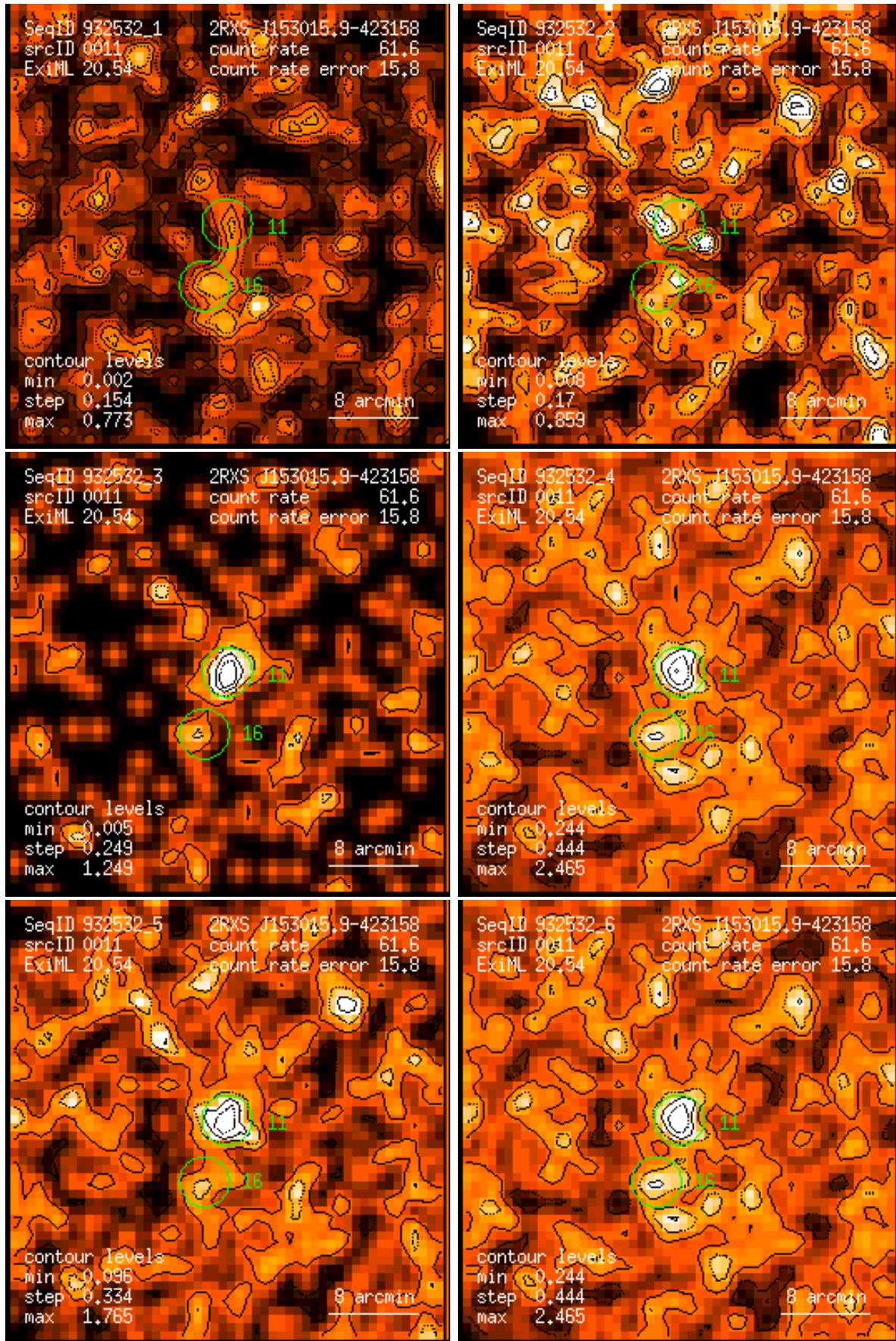
Figure 11: RASS 932532: detection 0011: band rate images, Gaussian filter: (1) PSPC channels 11 – 41, (2) 52 – 90, (3) 91 – 201, (4) 11 – 235, (5) 52 – 201, (6) 11 – 201. Broad band rates in counts/ks. Band rate contour levels in counts/ks/arcmin 2 .
