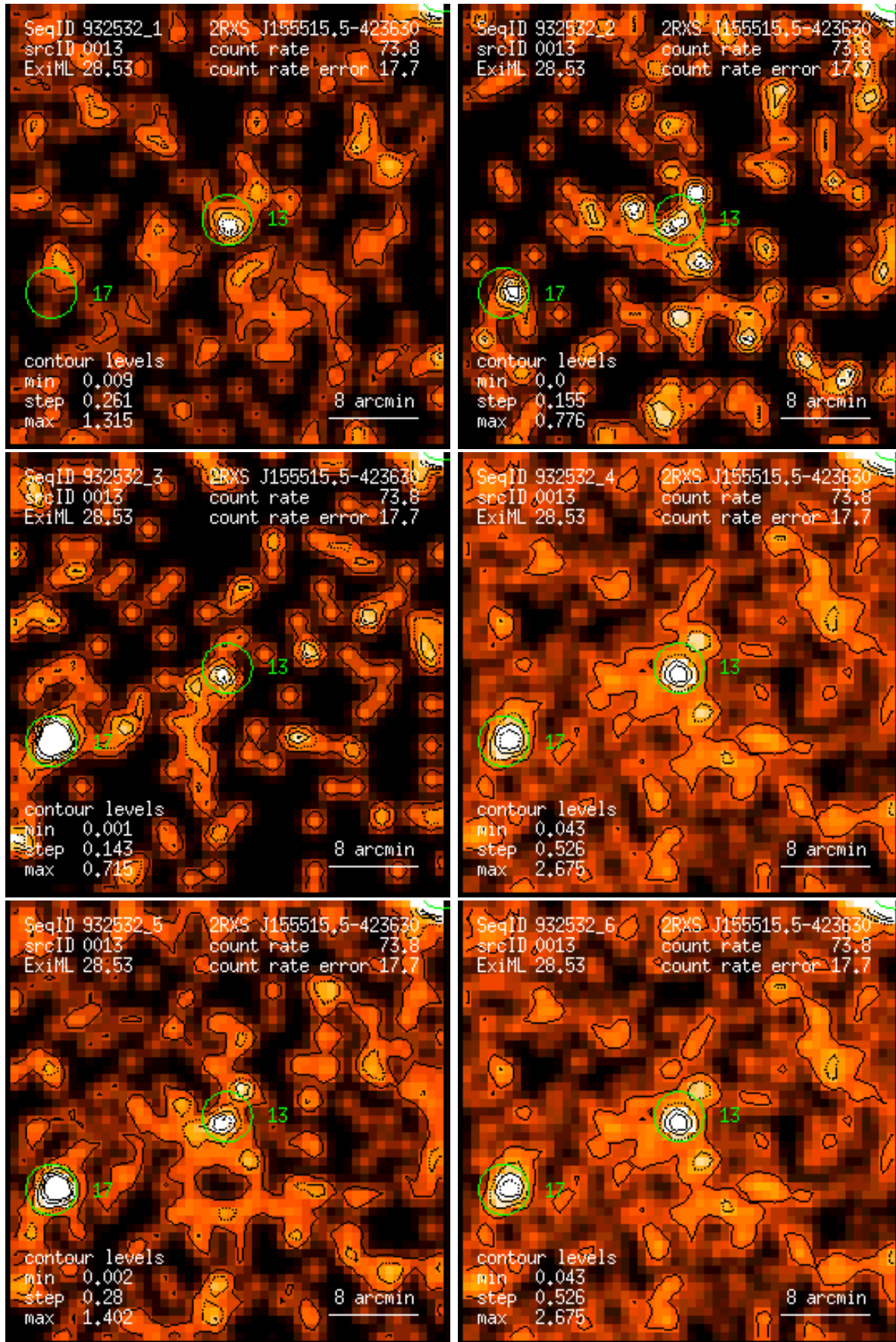
Figure 13: RASS 932532: detection 0013: band rate images, Gaussian filter: (1) PSPC channels 11 – 41, (2) 52 – 90, (3) 91 – 201, (4) 11 – 235, (5) 52 – 201, (6) 11 – 201. Broad band rates in counts/ks. Band rate contour levels in counts/ks/arcmin 2 .
