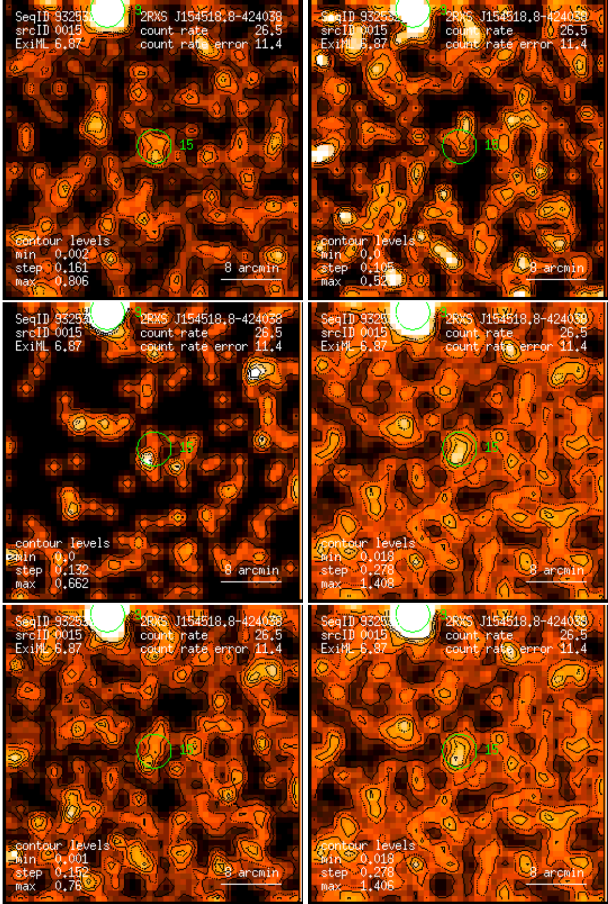
Figure 15: RASS 932532: detection 0015: band rate images, Gaussian filter: (1) PSPC channels 11 – 41, (2) 52 – 90, (3) 91 – 201, (4) 11 – 235, (5) 52 – 201, (6) 11 – 201. Broad band rates in counts/ks. Band rate contour levels in counts/ks/arcmin 2 .
