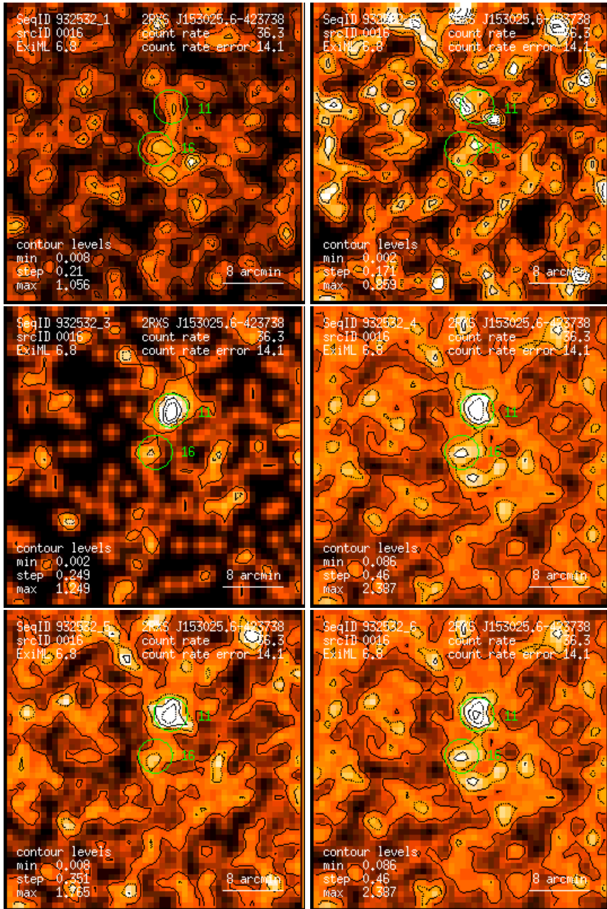
Figure 16: RASS 932532: detection 0016: band rate images, Gaussian filter: (1) PSPC channels 11 – 41, (2) 52 – 90, (3) 91 – 201, (4) 11 – 235, (5) 52 – 201, (6) 11 – 201. Broad band rates in counts/ks. Band rate contour levels in counts/ks/arcmin 2 .
