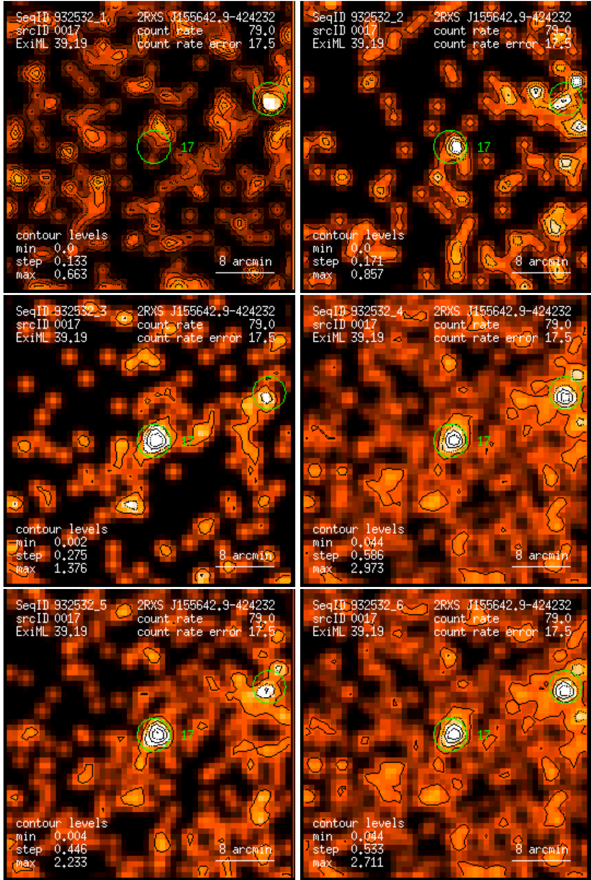
Figure 17: RASS 932532: detection 0017: band rate images, Gaussian filter: (1) PSPC channels 11 – 41, (2) 52 – 90, (3) 91 – 201, (4) 11 – 235, (5) 52 – 201, (6) 11 – 201. Broad band rates in counts/ks. Band rate contour levels in counts/ks/arcmin 2 .
